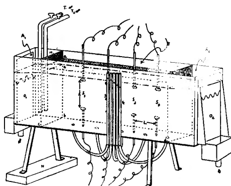
Fig. 1. Experimental apparatus. A_1 : supply tank; A_2 : drainage tank B : sand layer; N : pedestal M_1, M_2 : brass nets; T_1, T_2 : water pipes O_1, O_2 : movable walls S_1, S_2, S_3 and S_4 : cells; G : water manometers ab = 30.0\text{cm} ; bc = 10.0\text{cm} ; cd = 75.8\text{cm} ae = 4\sim 5.5\text{cm} ; l = 10\text{cm} ; L = 17.3\text{cm}
