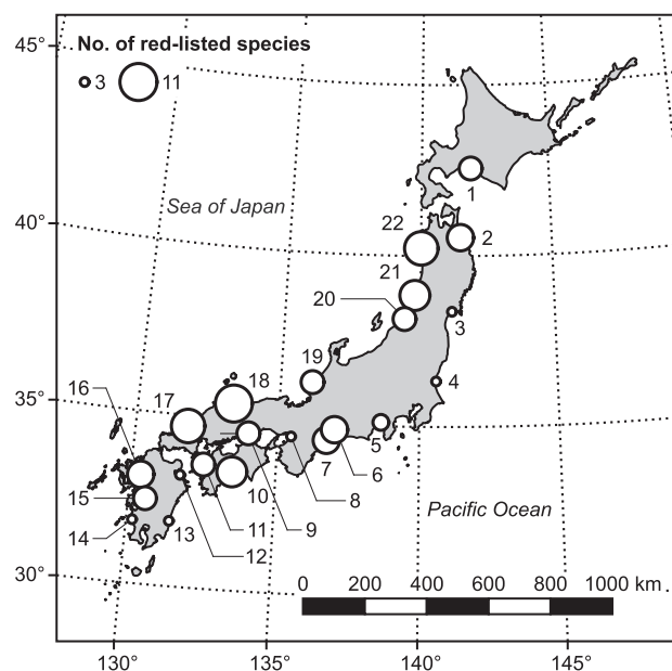
FIGURE 1 Map of water sampling locations in Japan. The size of circle is proportional to the number of fish species on the Japanese Red Lists detected at each site. Numbers are rivers: 1, Mukawa; 2, Mabechi; 3, Naruse; 4, Naka; 5, Fuji; 6, Yahagi; 7, Miyagawa; 8, Yamato; 9, Asahi; 10, Niyodo; 11, Hijikawa; 12, Onogawa; 13, Oyodo; 14, Sendai; 15, Kuma; 16, Chikugo; 17, Takatsu; 18, Hino; 19, Kuzuryu; 20, Arakawa; 21, Akagawa; 22, Yoneshiro
