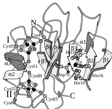
Figure 1. Schematic drawing of the Sulfolobus Fd molecule. \beta -strands are shown as gray arrows and \alpha -helices are shown as gray spirals. The [3Fe-4S] clusters, the seven cysteines, the zinc ion and the four zinc-ligand residues are represented as ball-and-stick models. Fe-S cluster I and II are indicated as I and II, respectively.
