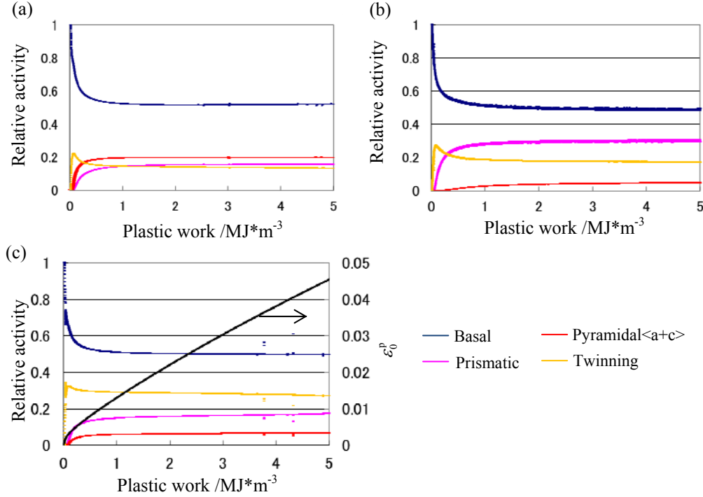
Fig. 8 Transition of relative activities under stress ratios of (a) 1:1, (b) -1:1, and (c) -1:-1.
