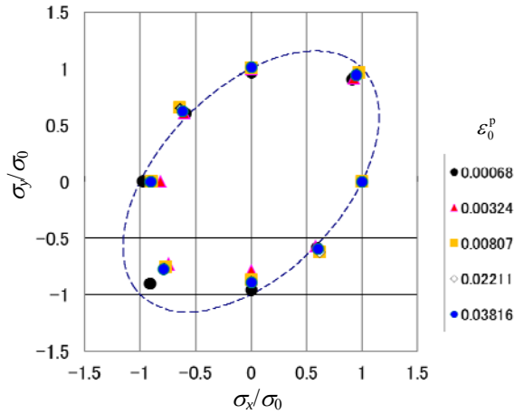
Fig. 7 Normalized contour of plastic work obtained from simulation. Contours are normalized using the uniaxial stress in the x direction \sigma_0 . The dotted line represents the von Mises yield locus. \varepsilon_0^p denotes the uniaxial plastic strain in the x direction.
