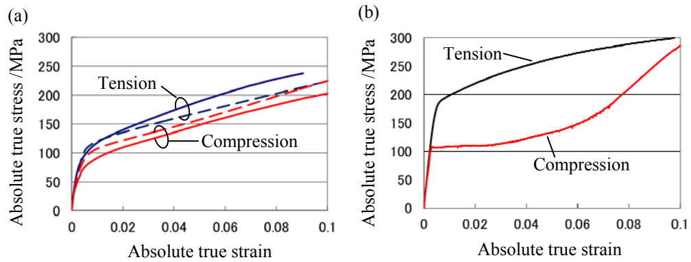
Fig. 3 Absolute true stress-absolute true strain curves obtained under uniaxial tension and compression. (a) Cast sheet and (b) rolled sheet. The solid and dotted lines are experimental and simulation results, respectively.
