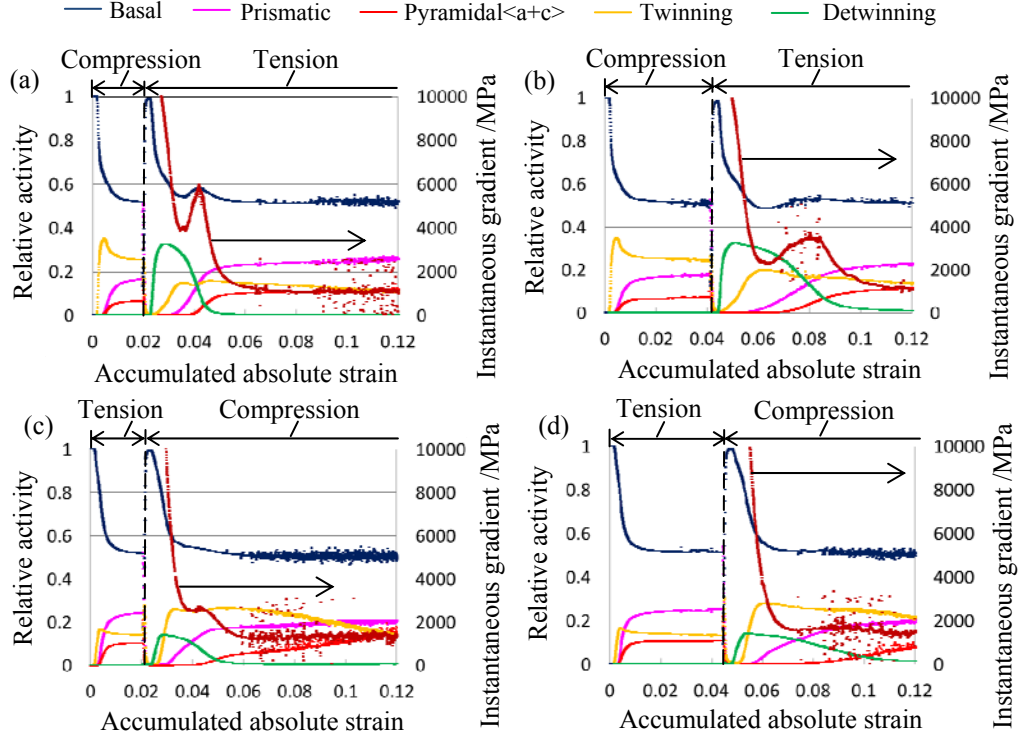
Fig. 6 Transition of relative activities during cyclic loading. (a) 2% CT, (b) 4% CT, (c) 2% TC, and (d) 4% TC.
