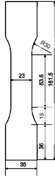
Fig. 2 Geometry of specimen in mm
