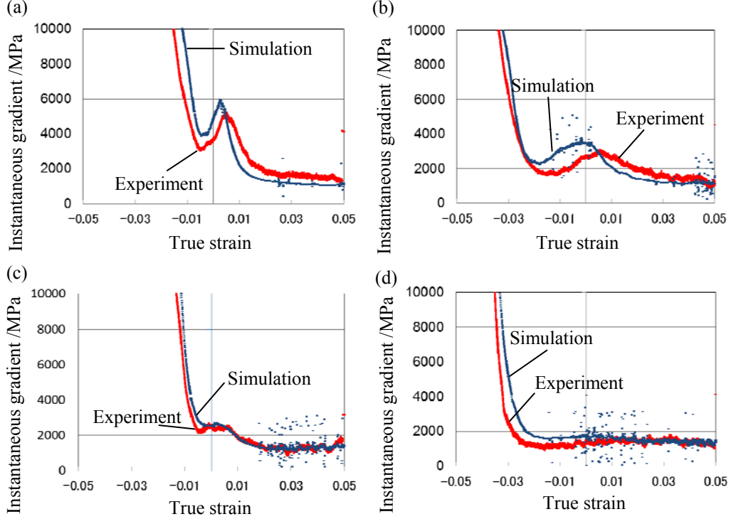
Fig. 5 Evolution of instantaneous gradient after the loading direction is inverted. (a) 2% CT, (b) 4% CT, (c) 2% TC, and (d) 4% TC. The signs of stress and strain in TC results are inverted.
