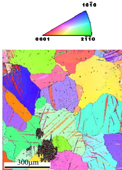
Fig. 1 Inverse pole figure of sample
