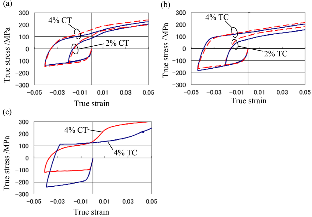
Fig. 4 True stress-true strain curves obtained under reverse loading tests. (a) CT results of cast sheet, (b) TC results of cast sheet, and (c) CT and TC results of rolled sheet. The solid and dotted lines are experimental and simulation results, respectively. The signs of stress and strain in TC results are inverted.
