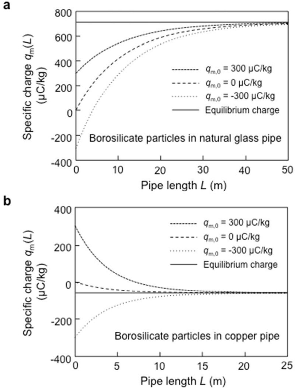
Figure 7. Predicting charging profile for borosilicate particles a) in natural glass pipe b) in copper pipe
