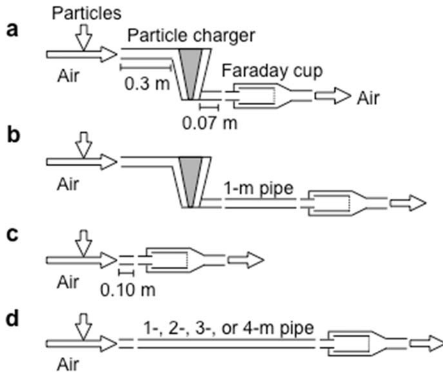
Figure 2. Experimental setup for determining a) initial particle charge after leaving the particle charger b) particle charge after 1-m pipe length c) particle charge leaving the ejector d) particle charge after different pipe lengths.
