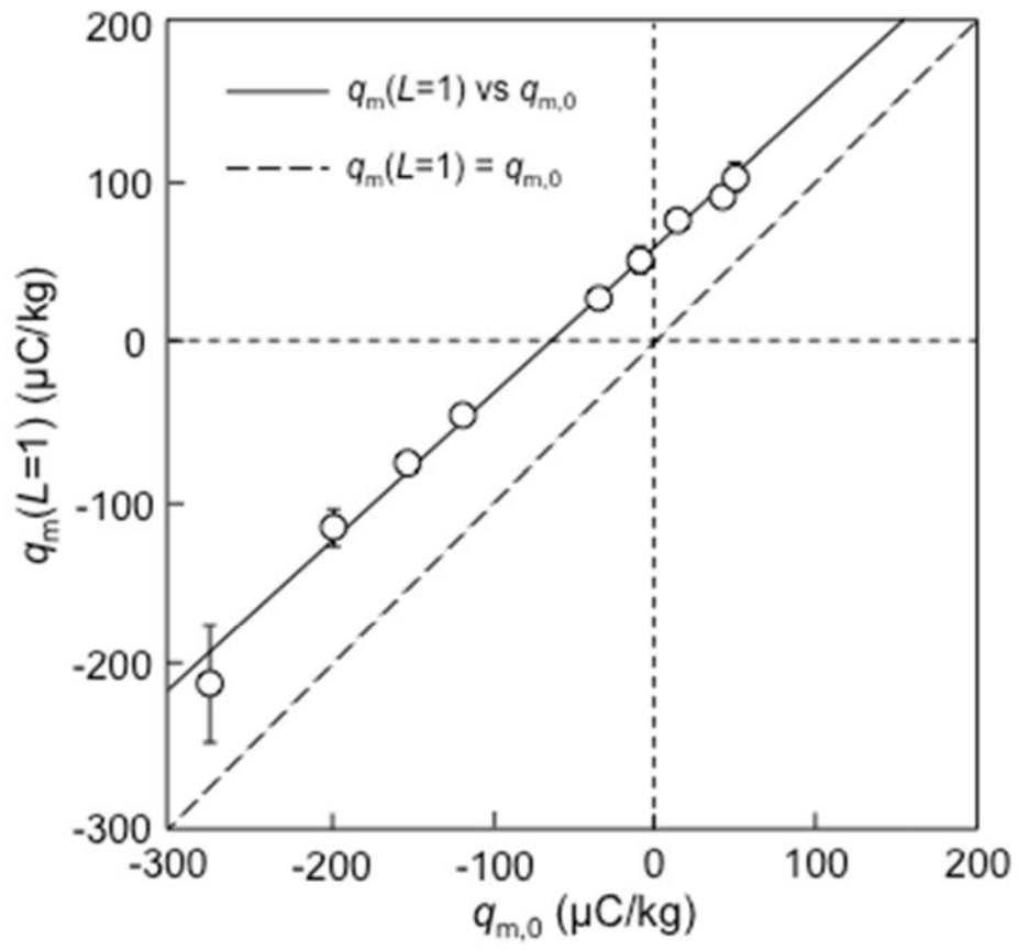
Figure 4. q_m(L = 1) vs. q_{m,0} for borosilicate particles in 1m natural glass pipe
