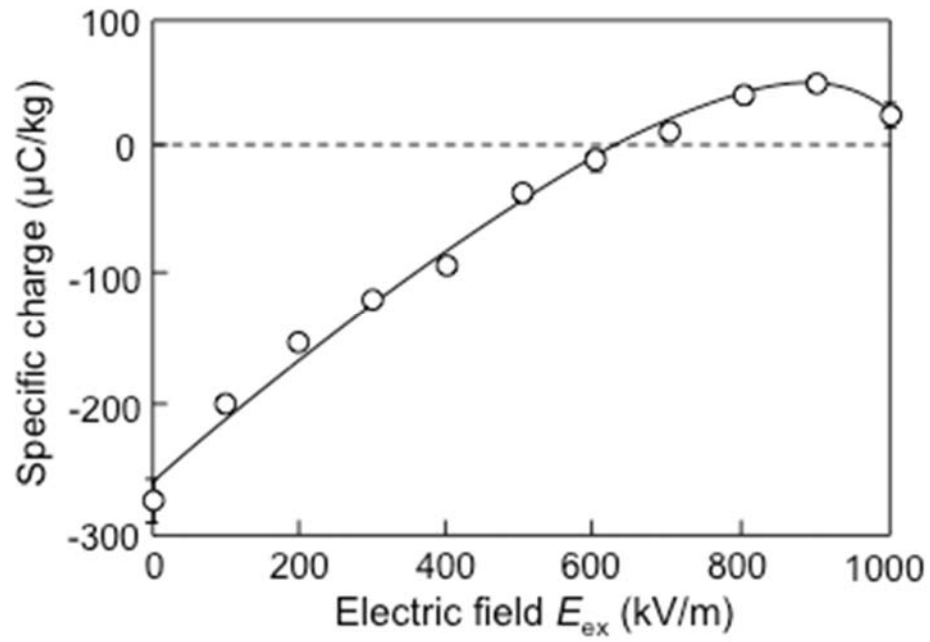
Figure 3. Specific charge of borosilicate particles leaving the particle charger as a function of applied electrical field in the particle charger.
