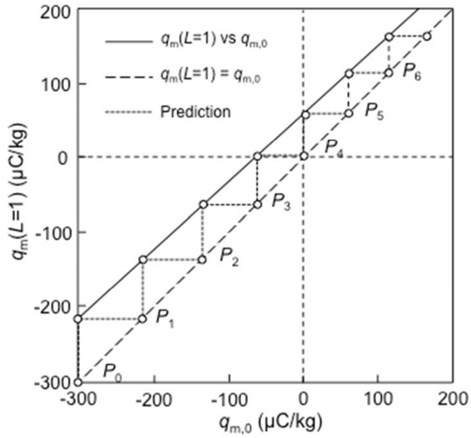
Figure 6. Predicting particle charge in natural glass pipe using stair-step method
