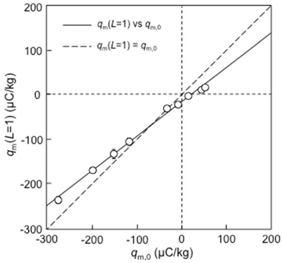
Figure 5. q_m(L = 1) vs. q_{m,0} for borosilicate particles in 1m copper pipe
