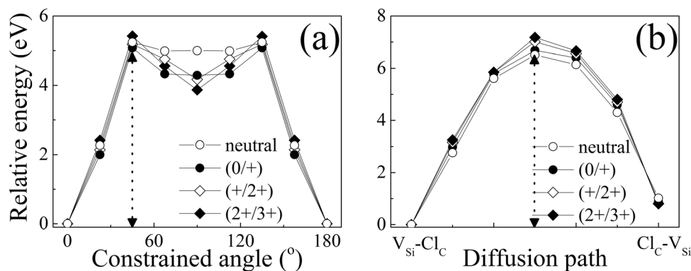
FIG. 4. Minimum energy path for (a) concerted exchange of \text{Cl}_C and C and (b) site change of \text{V}_{\text{Si}} by second neighbor hop of a Si atom, for the neutral, singly, doubly, and triply positive charge states of the \text{Cl}_C \text{V}_{\text{Si}} complex.
