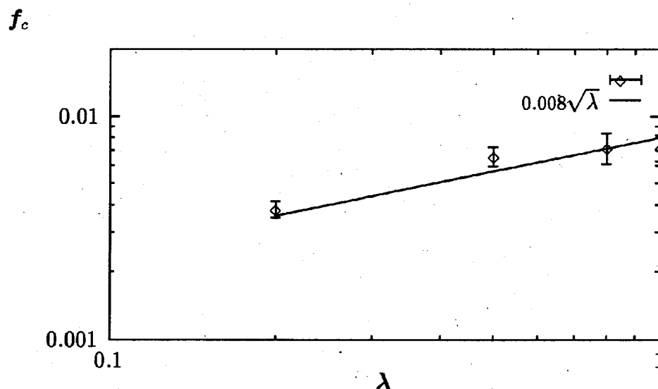
FIG. 2. The dependence of f_c on the non-linear parameter \lambda for N = 12 . We estimate the errorbar by sample average over five data of f_c . One datum of f_c is evaluated using a PSD already sample-averaged over ten PSDs with other initial conditions. The line represents the relation f_c \sim \sqrt{\lambda} . The experimental data is taken at \lambda = 0.2 \sim 1 from the second mode data. This result suggests that it is difficult to observe 1/f fluctuations in realistic phenomena which must have small non-linearity.
