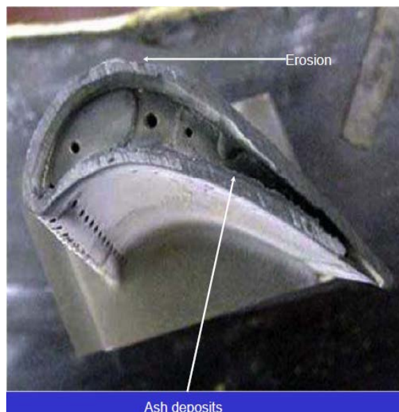
Fig. 3 Melted ash on turbine blade (Royo, 2010)
