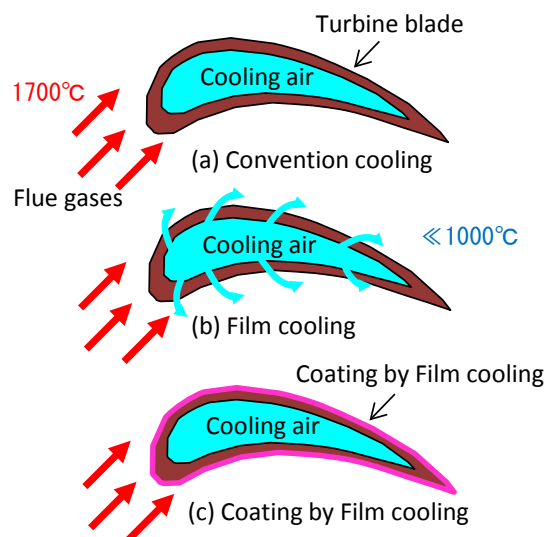
Fig. 2 Cooling of turbine blade
