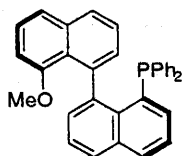
(R)-1
