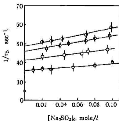
Fig. 6 Pseudo first-order rate constant, 1/\tau_2 , as a function of [\text{Na}_2\text{SO}_3]_0 at various ionic strength ( 25.0^\circ\text{C} ). Symbols represent the same as those in Fig. 5
