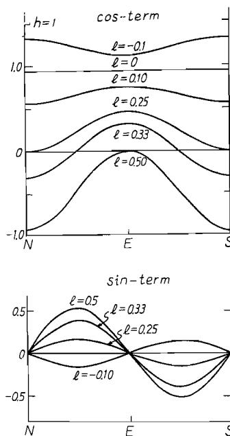
Fig. 3. The calculated coefficients of cos t -term and sin t -term of the tidal strain (for diurnal-component) vs. the azimuth.
