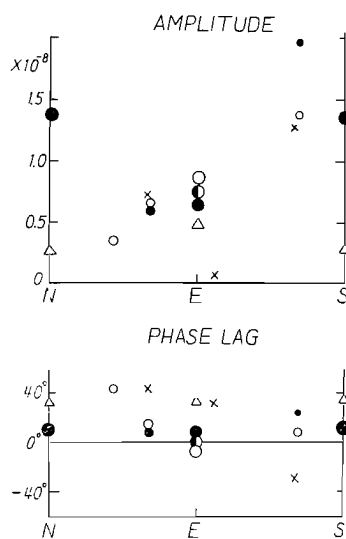
Fig. 1. Relation of amplitudes and phase lags of M_2 -constituent of linear strain vs. azimuth at Osakayama, Kishu and Matsushiro. \circ , \bullet , \bullet show the values, obtained from the observations at Osakayama, \times shows ones at Kishu, and \triangle shows ones at Matsushiro.
