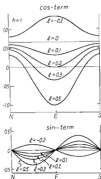
Fig. 2. The calculated coefficients of cos 2t -term and sin 2t -term of the tidal strain (for semi-diurnal component) vs. the azimuth.
