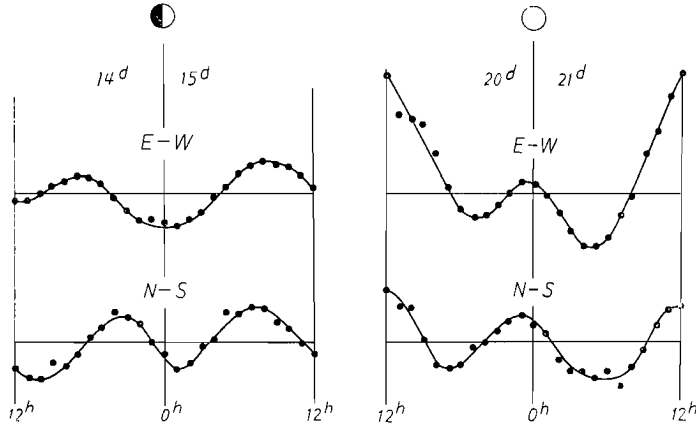
Fig. 4. Observed tide curves of the linear strains which are eliminated the secular changes, in the prime vertical component and in the meridional component at Osakayama on June 1959.
