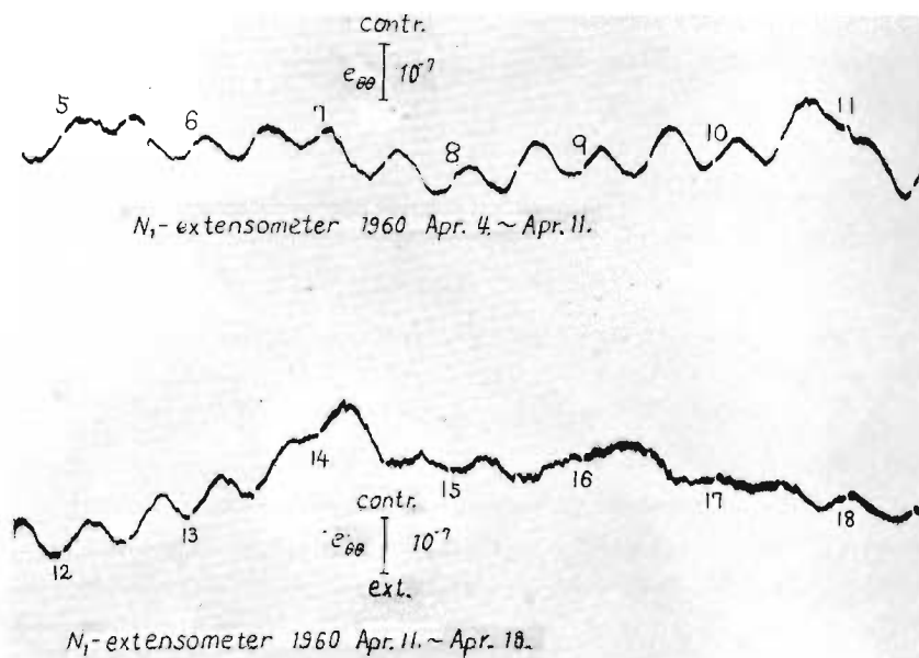
Photo 1 (a) and (b). The photographic tidegrams of linear strains which are recorded with the extensometers at Osakayama. e_{\theta\theta} and e_{\phi\phi} show the meridional and the prime vertical components of the ground-strains, respectively.
