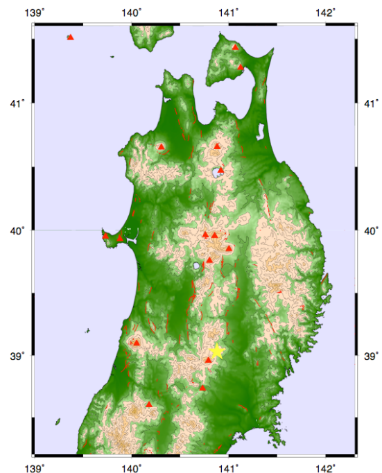
Fig. 1 Location of the epicenter (star) of 2008 Iwate-Miyagi Nairiku earthquake. Topography (GSI, 2002) is also shown with active volcanoes (triangles; Sibert and Simkin, 2002) and active faults (red lines; Research Group for Active Faults of Japan, 1980).
