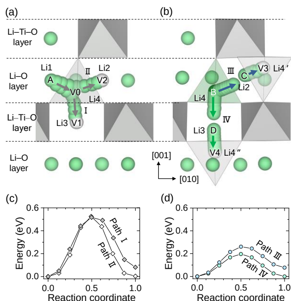
Figure 5. \text{Li}^+ ion migrations via (a,c) a vacancy mechanism and (b,d) an interstitialcy mechanism, which were investigated by DFT calculations and NEB method. (a) \text{Li}^+ ion migration paths I and II via the vacancy mechanism where a \text{Li}^+ ion A migrates from the Li1 site to vacant Li3 and Li2 sites, respectively, through a vacant Li4 interstitial site (Initial state of the migration along the path I: A at Li1 site, vacancy V0 at Li4 site, vacancy V1 at Li3 site; Final state of the migration along the path I: V0 at Li1 site, V1 at Li4 site, A at Li3 site; Initial state of the migration along the path II: A at Li1 site, V0 at Li4 site, V2 at Li2 site; Final state of the migration along the path II: V0 at Li1 site, V2 at Li4 site, A at Li2 site). (b) \text{Li}^+ ion migrations along paths III and IV via the interstitialcy mechanism where an interstitial \text{Li}^+ ion B pushes (kicks) another \text{Li}^+ ion at a lattice site (C for the path III; D for the path IV) out into an adjacent vacant interstitial site. In the path III, the B moves from Li4 to Li2 site and simultaneously another \text{Li}^+ ion C migrates from Li2 to vacant Li4' site (Initial state: B at Li4 site, C at Li2 site, a vacancy V3 at Li4' site; Final state: V3 at Li4 site, B at Li2 site, C at Li4' site). In the path IV, a Li ion B moves from Li4 to Li3 site and simultaneously another Li ion D migrates from Li3 to vacant Li4'' site (Initial state: B at Li4 site, D at Li3 site, V4 at Li4'' site; Final state: V4 at Li4 site, B at Li3 site, D at Li4'' site). Energy barrier profiles along the paths I and II (c) and along the paths III and IV (d).
