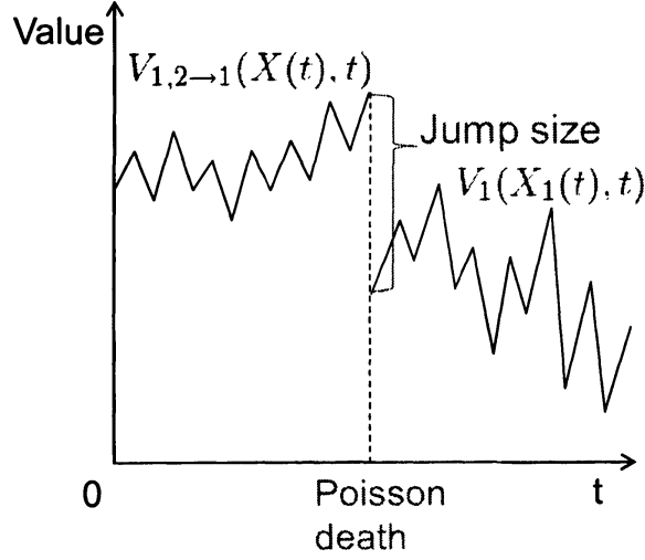
Figure 1: The downward jump caused by the disappearance of the alternative.
