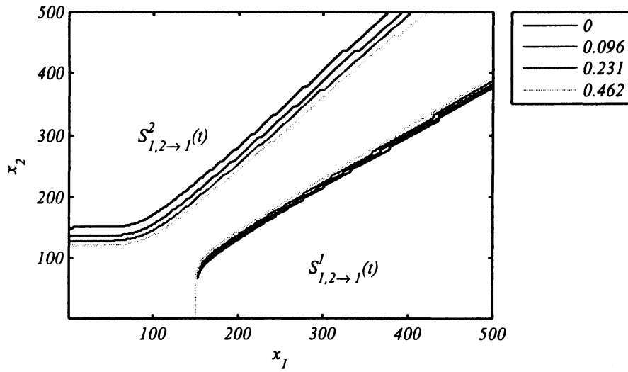
Figure 4: The exercise regions for the max-option that will change to the standard option. This figure plots the boundaries of the exercise regions S_{1,2 \rightarrow 1}(t) = S_{1,2 \rightarrow 1}^1(t) \cup S_{1,2 \rightarrow 1}^2(t) for the intensity \lambda = 0, 0.096, 0.231 , and 0.462 . For \lambda = 0 , the region is equal to the exercise region for the max-option, S_{1,2}(t) . The parameter values are set at the base case (1).
