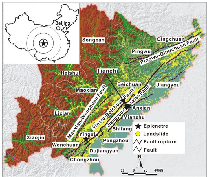
Fig. 1 Epicenter of Sichuan earthquake, distribution of landslides, and location of Tianchi landslide dam (after Huang and Li (2009)).
