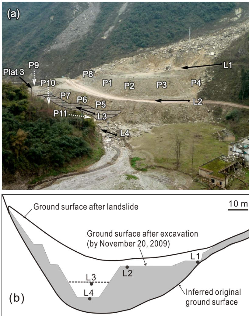
Fig. 6 (a) Photo of landslide dam after excavation with locations of S-wave survey lines and grain size analysis points (P1~P11); (b) Cross section of the landslide dam during differing surveying times. L3, L4: spillway levels on November 20, 2009, and June 16, 2010, respectively.
