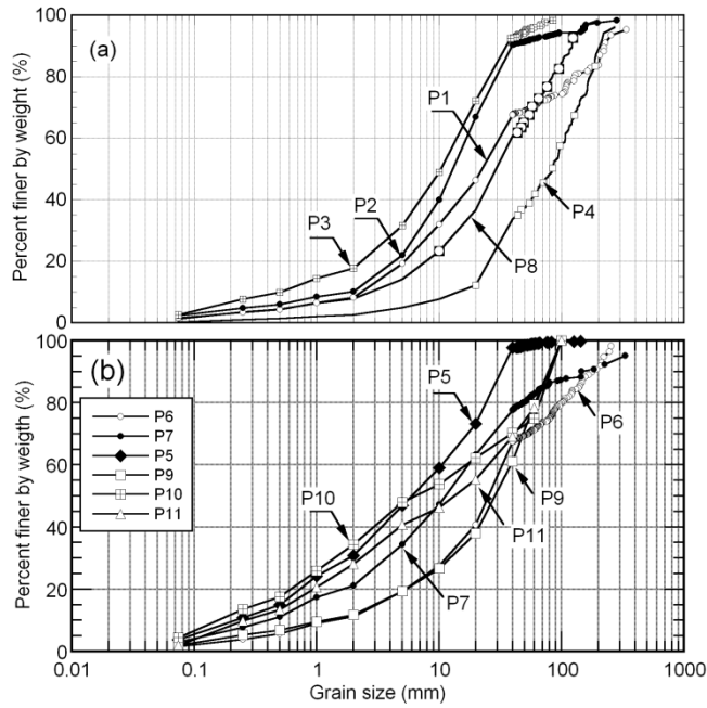
Fig. 7 Grain size distributions of materials from dam body. (a): samples on the same altitude level. (b): Samples at different depth of the dam body
