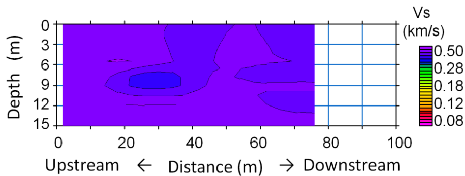
Fig. 9 Shear-wave velocity ( V_s ) profile along traverse line L1
