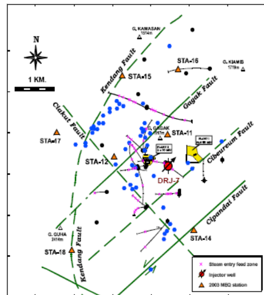
Fig. 12 Micro earthquakes distribution in 1997 and faults around Darajat geothermal field and (Pramono and Colombo, 2005)
