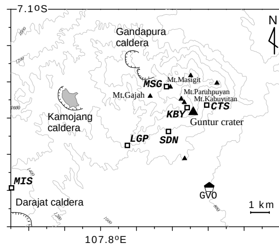
Fig. 1 Locations of seismic stations at Guntur volcano. Squares indicate seismic stations and triangles show peak of cones. GVO is Guntur Volcano Observatory.
