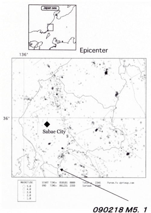
Fig. 1 Recent seismicity in Reiho region. From '01 Jan. to '06 Dec.. M is greater than 1.0. H is less than 30km.
