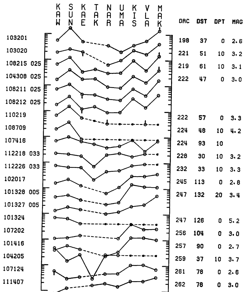
Fig. 3(c). See legend Fig. 3(a).
