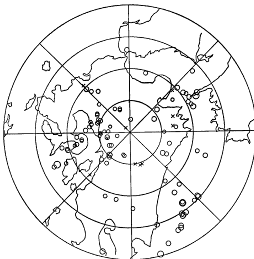
Fig. 2. Epicenters of earthquakes used in this analysis.
