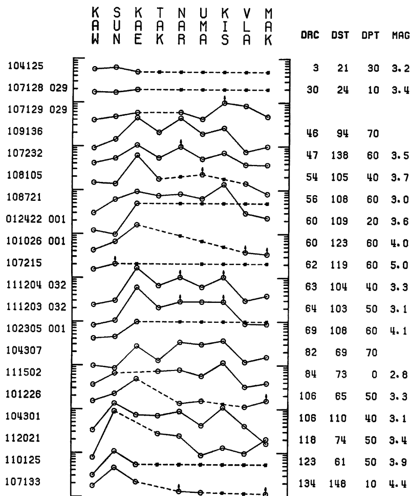
Fig. 3(a). Maximum amplitudes of P waves.
