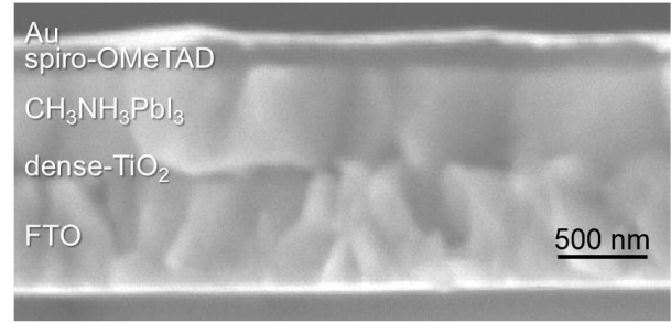
Fig. 3. A cross-sectional SEM image of a perovskite solar cell prepared from 55 wt% \text{CH}_3\text{NH}_3\text{PbI}_3 solution. The scale bar corresponds to 500 nm in length.
