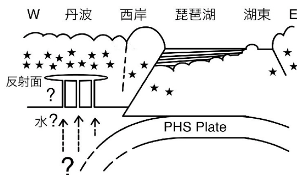
Fig. 9 schematic structure model across the Tamba and Oumi region
