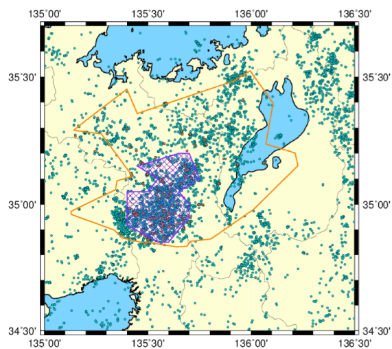
Fig. 4 Distribution of S-wave reflector in the lower crust. The reflector exists within the area shown by the purple mesh. (Aoki, 2013)
