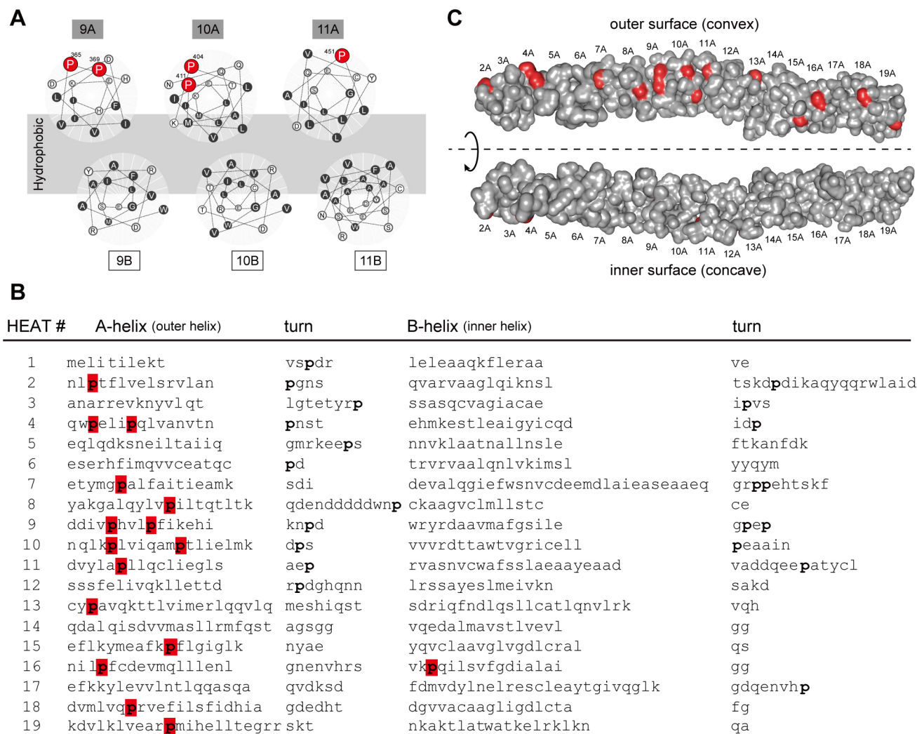
Fig. 1. Localization of proline residues in the convex surface of importin-β. (A) Top view of HEAT motifs 9, 10 and 11. Importin-β contains 19 HEAT repeats, which are composed of two amphiphilic α-helices (A-helix and B-helix) facing each other by hydrophobic interactions. Red: proline; gray: hydrophobic amino acid. (B) Positions of the proline residues in mouse importin-β1. The amino acid sequence of mouse importin-β1 is shown by aligning the 19 HEAT repeats. Proline residues in the α-helices (A-helix and B-helix) are indicated by bold and highlighted in red. (C) Surface representation of mouse importin-β based on its crystal structure (PDB: 1ukl). Only the A-helices are presented here (loops and B-helices are removed). All helices are aligned so they fit the same plane. Proline residues are indicated in red.
