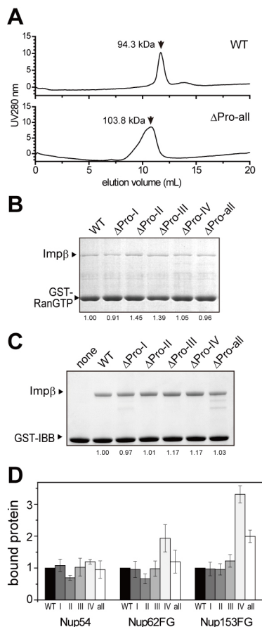
Fig. 5. Molecular properties of wild-type and mutant importin- \beta . (A) The elution profiles of wild-type (top graph) and \Delta Pro-all mutant (bottom graph) importin- \beta by gel filtration. On the basis of the elution profiles of the molecular markers (not shown here), the molecular masses of wild-type and mutant importin- \beta were estimated to be 94.3 and 103.8 kDa, respectively. (B) Binding assay of importin- \beta to RanGTP. GST-RanGTP was immobilized on beads and wild-type and mutated importin- \beta were added. An SDS-PAGE gel stained with Coomassie Brilliant Blue (CBB) is shown. The bands corresponding to importin- \beta and Ran are indicated by arrowheads. The relative amounts of importin- \beta bound to Ran-GTP were quantified and are presented below the gel. (C) Binding assay of importin- \beta to the IBB. GST-IBB was used for this assay. An SDS-PAGE gel stained with CBB is shown. The bands corresponding to importin- \beta and the IBB are indicated by arrowheads. The relative amounts of importin- \beta bound to IBB were quantified and are presented below the gel. (D) Results of the binding assay with Nups. Full-length Nup54, FG-repeat regions of Nup62 (amino acid residues 1–178) and Nup153 (896–1475) were used for the assay. The relative amounts of importin- \beta bound to the Nups immobilized on beads were quantified and are shown in the graph (bars: \pm s.d., n=3 ).
