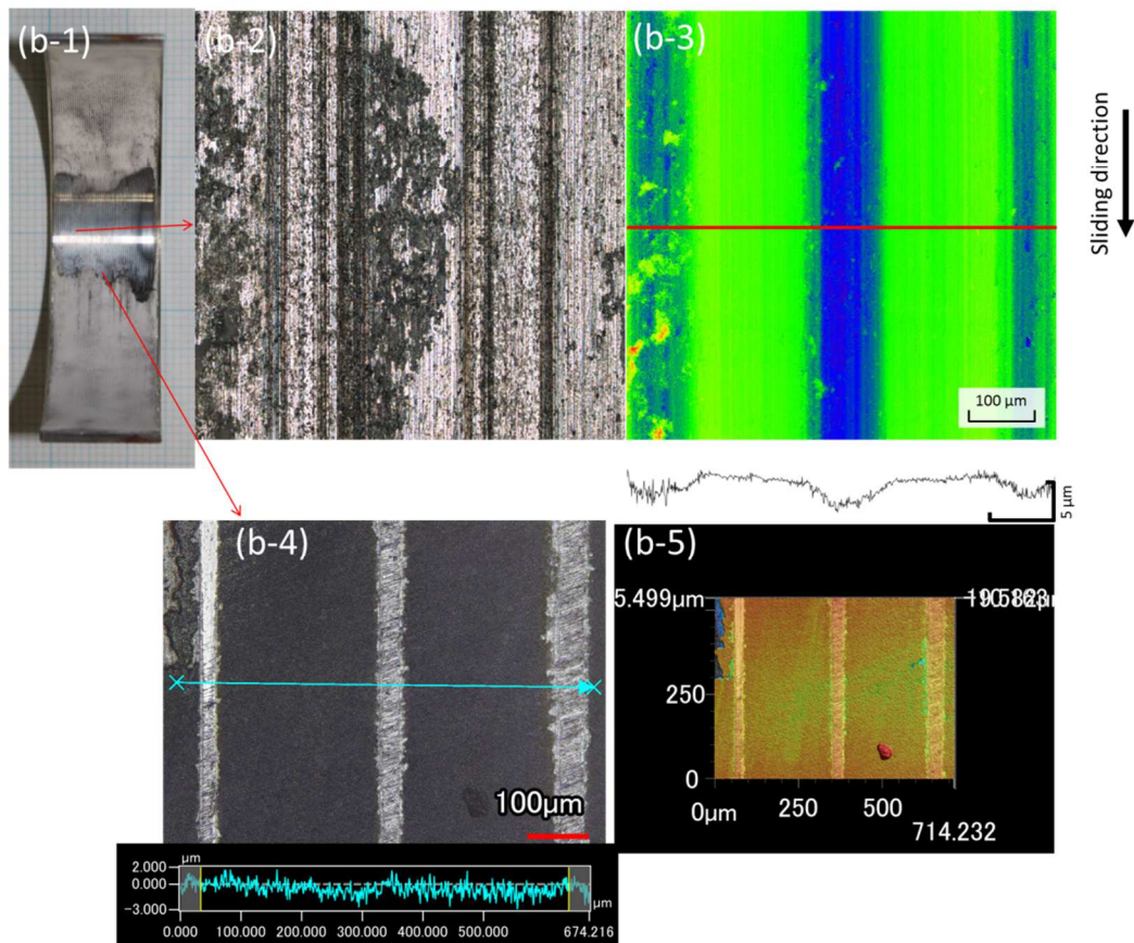
Figure 8-7. Appearance, laser microscopic images and surface roughness profiles of (a) a grooved bearing and (b) a monolith-coated bearing washed with hexane after tribological measurement by increasing loading in a stepwise. Arrows show the regime of observation.
