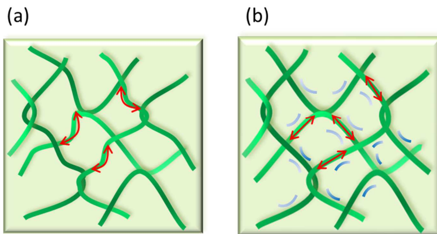
Figure 5-2. Illustration of behavior of network embedded in matrix. (a) bending-dominated deformation and (b) stretch-dominated deformation.
