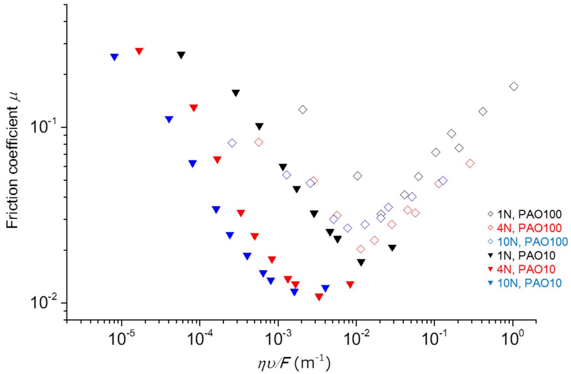
Figure 7-5. Plots of friction coefficient \mu against characteristic parameter \eta v/F for Al-coated monoliths prepared at 130 °C versus a Cr-SiO 2 -coated lens with PAO10 (closed triangles) and PAO100 (open diamonds).
