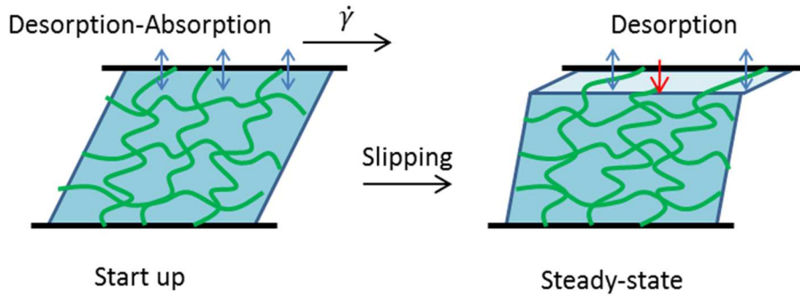
Figure 4-10. Illustration of transition from start-up-state to steady-state for the gel.
