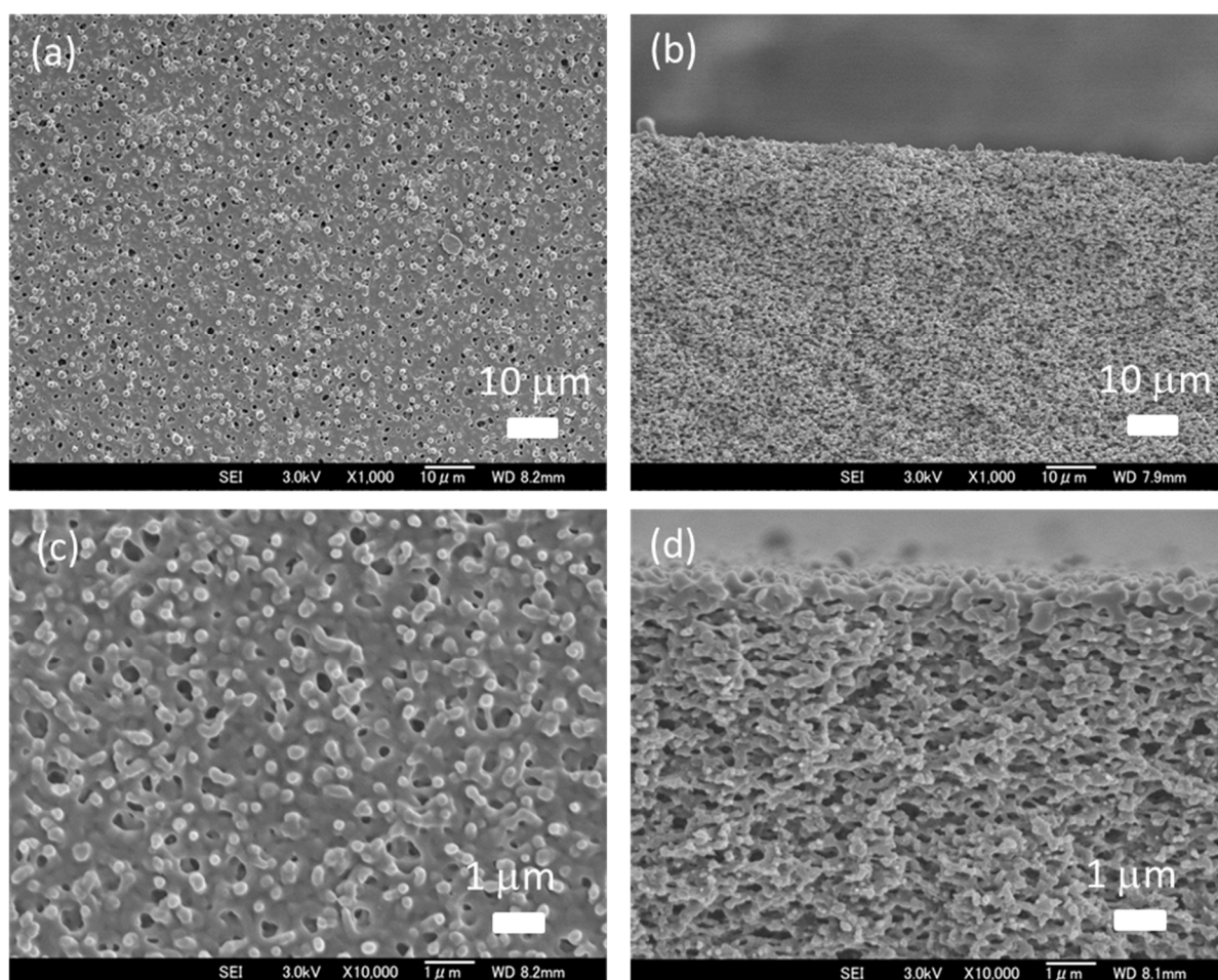
Figure 7-4. FE-SEM images of monoliths prepared by PVA-laminate method. Top-surface and cross-section of monoliths with a 170 \mu\text{m} in thickness (a),(b) at 100°C and (c),(d) at 130°C.
