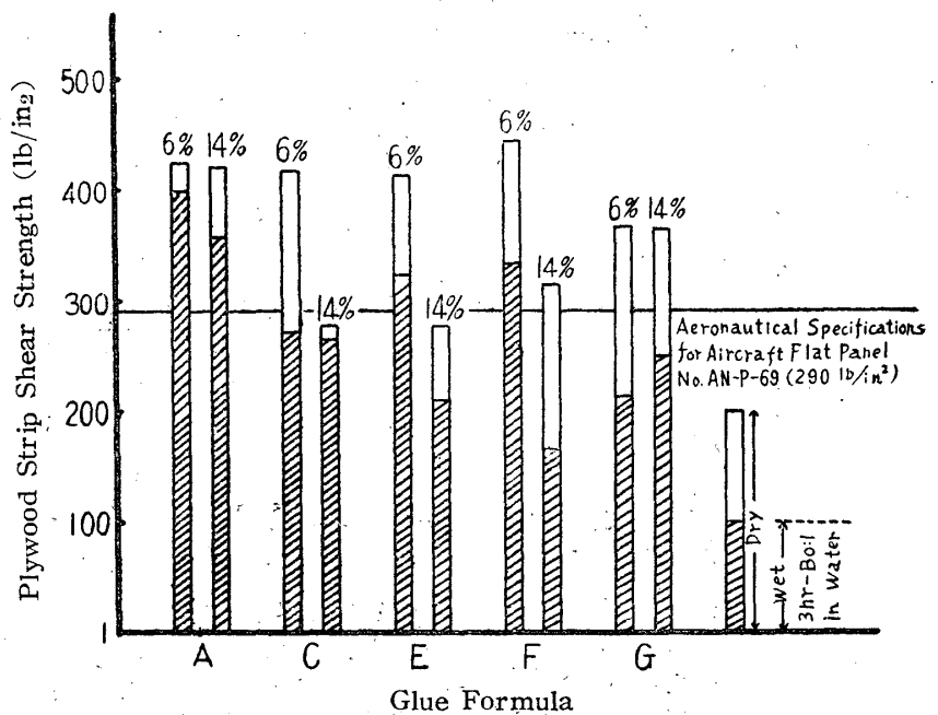
Fig.3 ; Influence of Moisture Content in Birch Veneer on Plywood Strip Shear Strength
