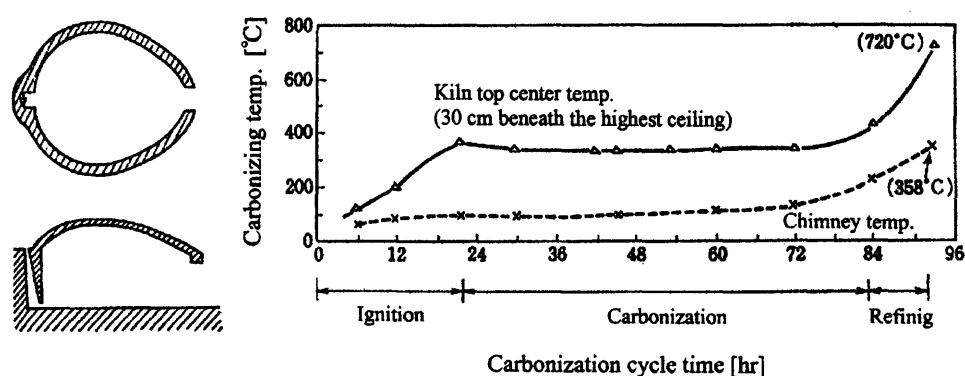
Fig. 4. Kurosumi kiln (Miura standard kiln) and its carbonizing temperature curves 5) .
