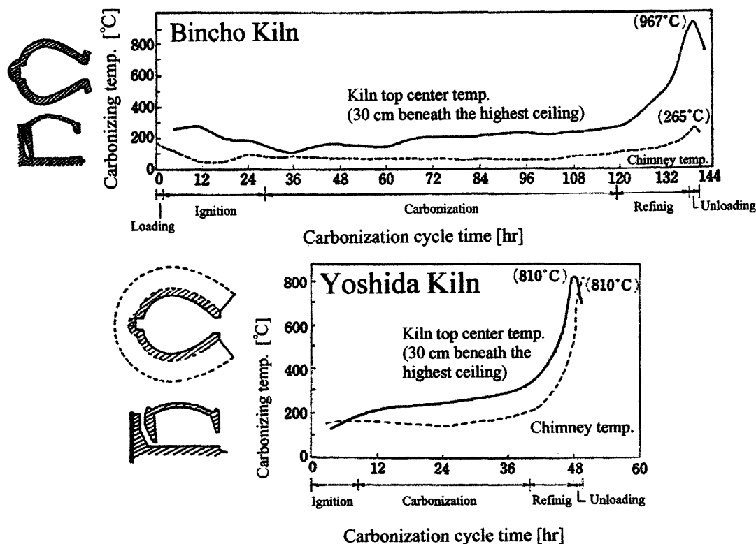
Fig. 5. Shirosumi kiln and its carbonizing temperature curves 5) .
