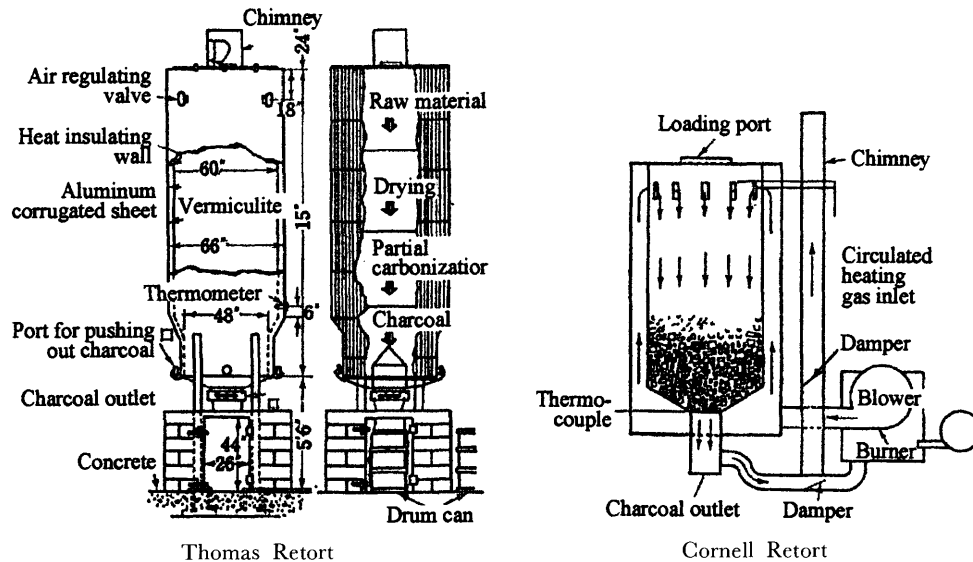
Fig. 6. Typical plants of dry distillation 5) .
