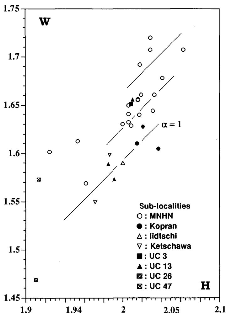
Fig. 13. Maximum width plotted against maximum height (hength) of Calcanei in Maragheh hipparions. Logarithmic scale. Hypothetical isometric growth lines were drawn for each morphotypes.
