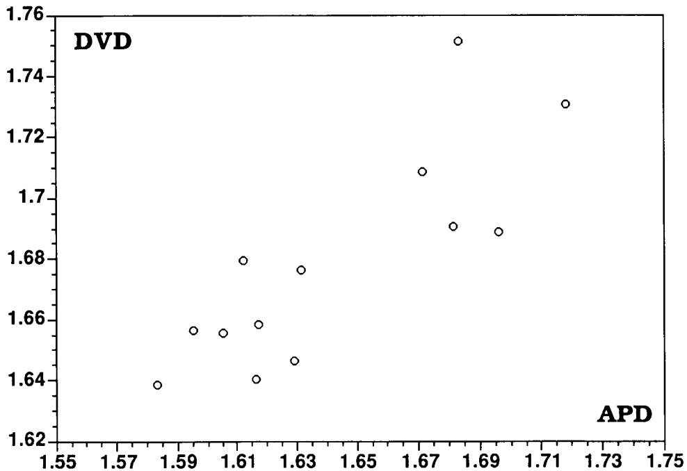
Fig. 14. Dorsoventral diameter of the acetabulum plotted against craniocaudal (anteroposterior) diameter in the Pelvic bone from Maragheh. Logarithmic scale. Two groups are distinguished by overall size. Small forms are probably of H. moldavicum . All samples belong to Kyoto University.
