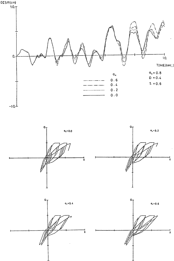
Fig. 35 Comparison of time histories of disp. (upper), comparison of hysteretic responses (X: disp., Q: shear forces) (lower) by the values of a_s
