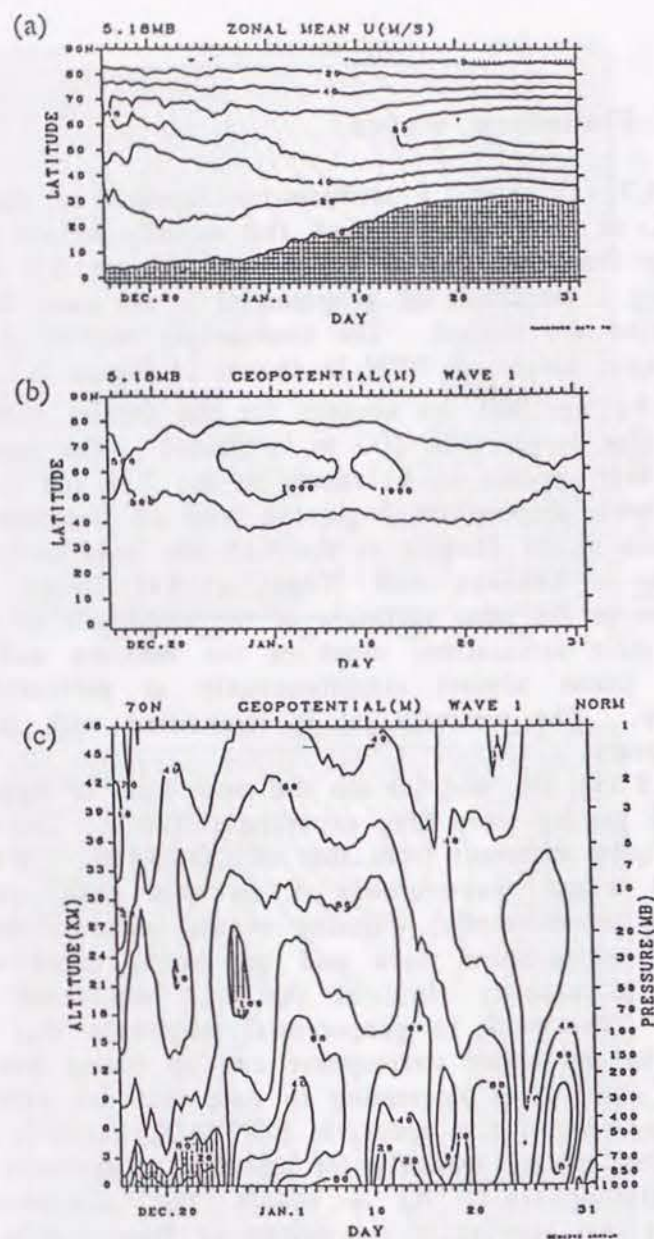
Figure 3.7: (a) Latitude-time section at 5.18 mb of the zonal wind ( 20 \text{ ms}^{-1} contours) for CONTROL( \kappa=0 ). Negative values are shaded. (b) Latitude-time section at 5.18 m of wave-1 amplitude of geopotential height (m). (c) Time-height section of wave-1 amplitude of geopotential height multiplied by \sqrt{p/1000} at 70^\circ\text{N} . Values larger than 100 are shaded.
