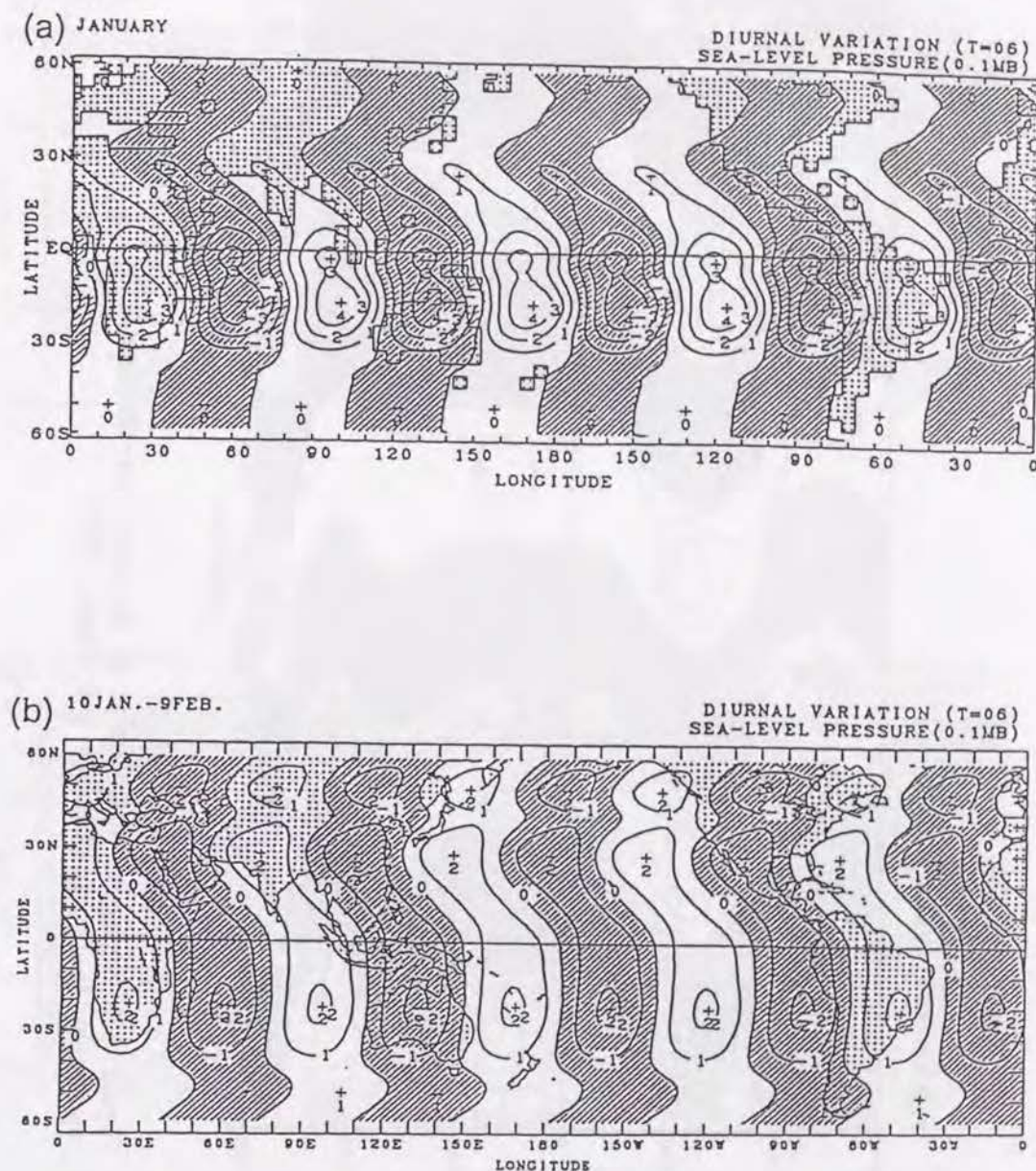
Figure 4.7: The horizontal map of sea level pressure field of the diurnal mode (f=-1, m=5) at 0600 GMT from (a) the GCM simulation and (b) FGGE IIIb(SOP-1) data analysis. The contour interval is 0.1 mb, and negative values are shaded.
