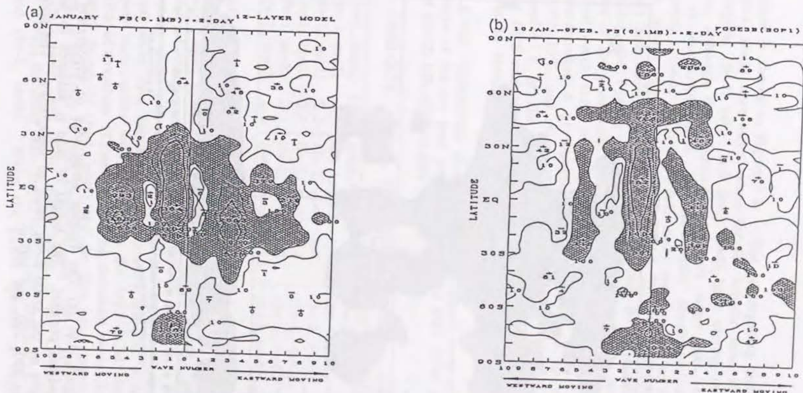
Figure 4.6: (a) The power spectra of the sea level pressure field in the latitude-wavenumber domain from the GCM simulation. The contours are 10, 100, 500, and 1000 (0.1 \text{ mb})^2 \text{ day}^{-1} . Values larger than 100 are shaded. (b) Same as Figure 4.6(a) except for FGGE IIIb(SOP-1) data analysis.
