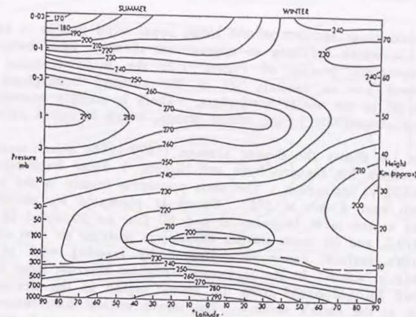
Figure 1.2: Schematic latitude-height section of zonal mean temperatures (K) at the solstices [Murgatroyd, 1969].
