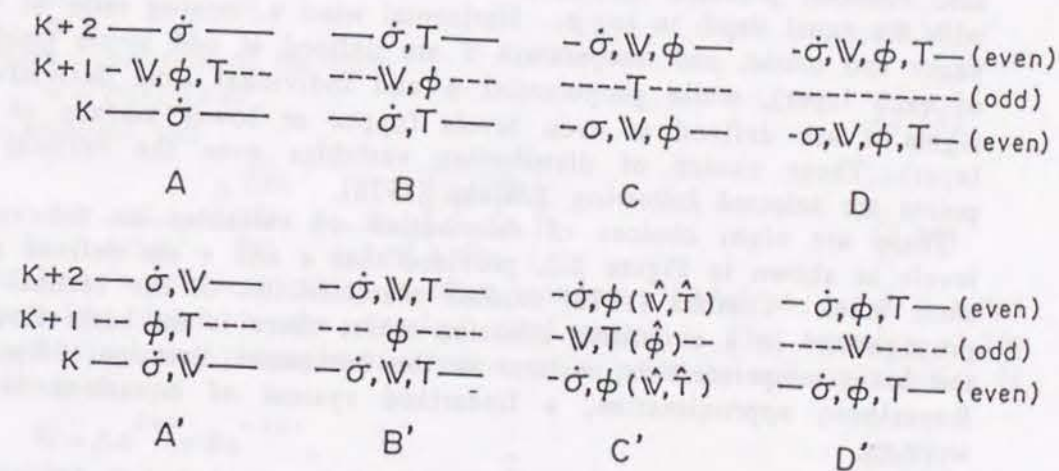
Figure 2.2: Eight choices of distributing variables on vertical levels. ^ is a reminder that the variable is an interpolated value from the non-hat ones. Scheme C' is adopted in the MRI GCM-I [Tokioka et al. , 1984].
