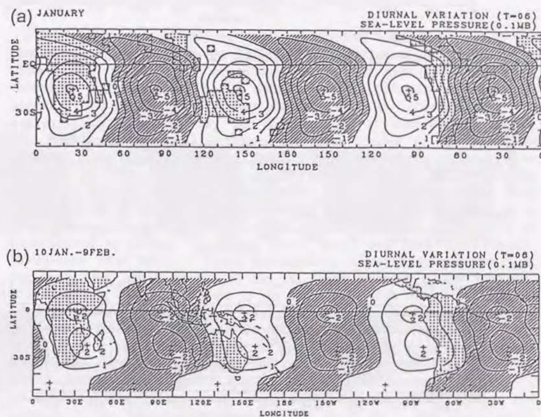
Figure 4.11: The same as in Fig.4.7 but for the mode ( f=1 , m=3 ).
