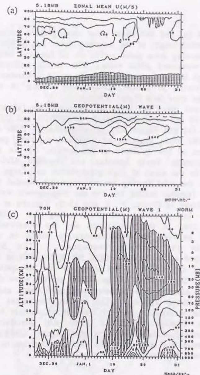
Figure 3.8: (a) Latitude-time section at the 5.18 mb level of the zonal wind ( 20 \text{ ms}^{-1} contours) for the gravity wave drag experiment IGW/6. Negative values are shaded. (b) Latitude-time section at 5.18 m of wave-1 amplitude of geopotential height (m). (c) Time-height section of wave-1 amplitude of geopotential height multiplied by \sqrt{p/1000} at 70^\circ\text{N} . Values larger than 100 are shaded.
