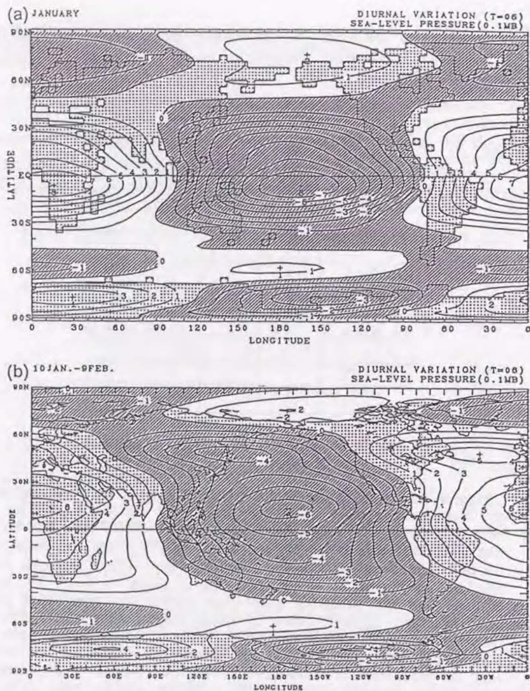
Figure 4.2: The horizontal map of sea level pressure field of the diurnal mode ( f=-1 , m=1 ) at 0600 GMT from (a) the GCM simulation and (b) FGGE IIIb(SOP-1) data analysis. The contour interval is 0.1 mb, and negative values are shaded.
