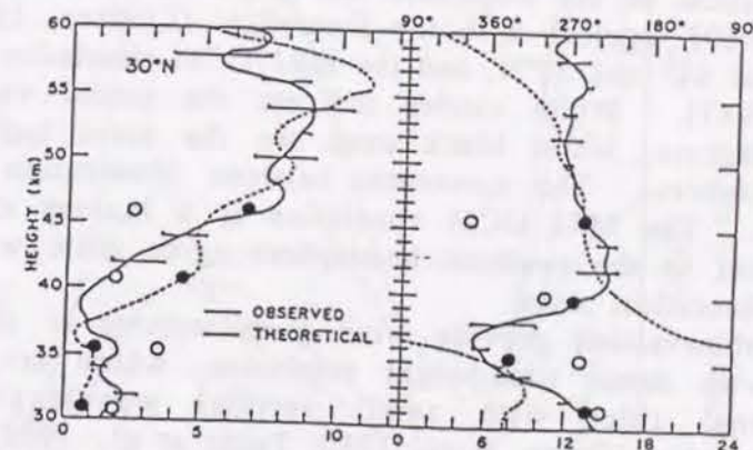
Figure 1.11: The vertical distribution of the amplitude (left) and phase (right) of meridional wind for the westward moving wavenumber 1 diurnal tide at 61°N (top) and 30°N (bottom). The results by the MRI GCM are plotted by circles on the figure reproduced from Reed et al. (1969). White and black circle indicate the values at the nearest grid points to 61° and 30° in the northern and southern hemispheres, respectively. The solid line shows the results by Reed et al. (1969), the dashed line by Lindzen (1967) and the thin solid line by Forbes (1982a) [Tokioka and Yagai, 1987].
