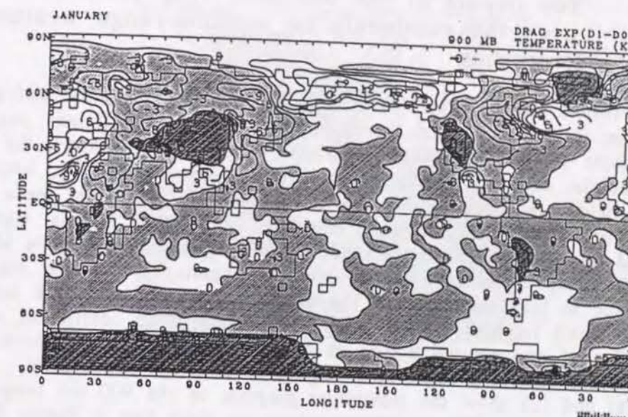
Figure 3.18: The 30-day averaged difference, D_1-D_0 , of the temperature at the 900 mb level. The contour interval is 3^\circ\text{K} and negative values are shaded.
