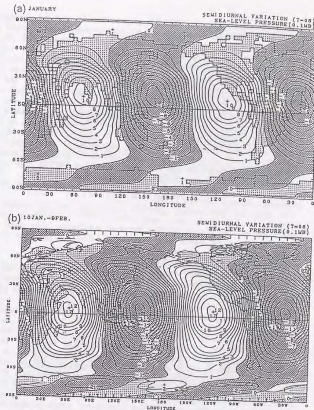
Figure 4.3: The horizontal map of sea level pressure field of the semi-diurnal mode ( f=-2 , m=2 ) at 0600 GMT from (a) the GCM simulation and (b) FGGE IIIb(SOP-1) data analysis. The contour interval is 0.1 mb, and negative values are shaded.
