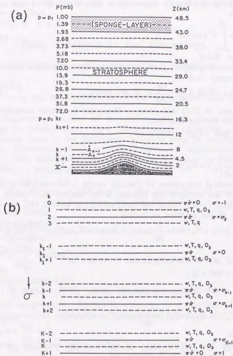
Figure 2.1: (a) The vertical discretization of the twelve layer version of the MRI GCM-I. (b) The vertical indices and the position of vertical levels for the model [Arakawa and Lamb, 1977]. Solid and dashed lines indicate even and odd levels, respectively. The lowest odd level is indicated as K. Approximate positions of the levels in km are shown when the surface pressure is 1000 mb.
