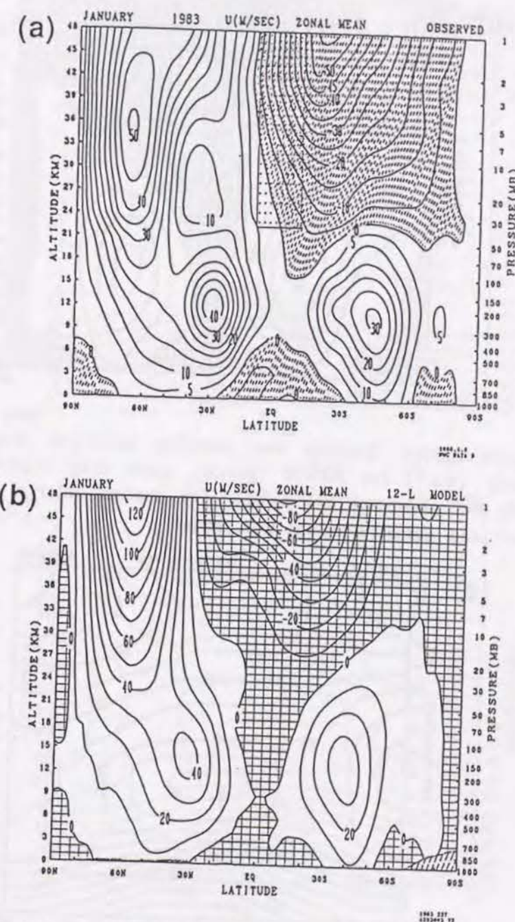
Figure 3.3: Zonally and monthly averaged westerly winds ( \text{ms}^{-1} ) for (a) January analysis for the year 1983 and (b) the CONTROL simulation. The contour interval is 5 \text{ ms}^{-1} in the observation and 10 \text{ ms}^{-1} in the simulation. Negative values are shaded.
