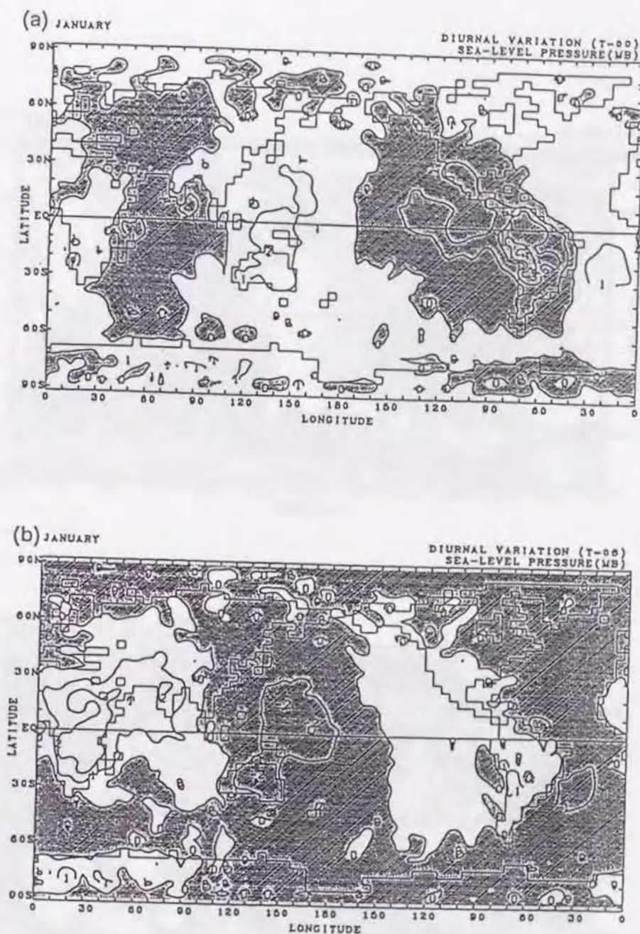
Figure 4.4: Diurnal variation of sea level pressure field at 0000, 0600, 1200, and 1800 GMT from the GCM simulation ((a), (b), (c), and (d)) and FGGE IIb(SOP-1) data analysis ((e), (f), (g), and (h)). The contour interval is 1.0 mb, and negative values are shaded.
