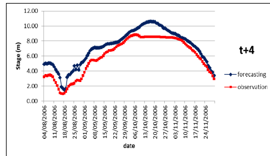
Fig. 26 Forecasting result of C.7A at time t+4
