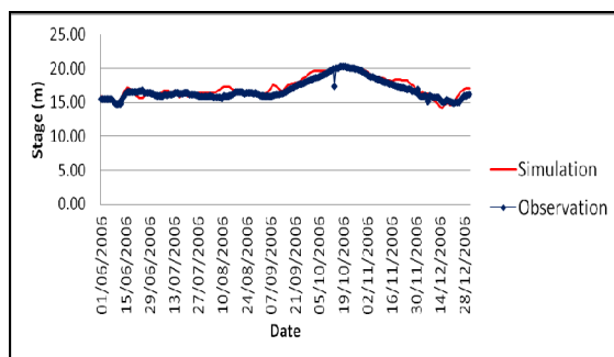
Fig. 5 Calibrated result at Manorom
