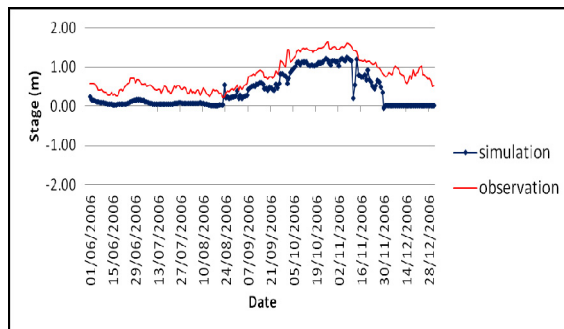
Fig. 10 Calibrated result at Memorial Bridge
