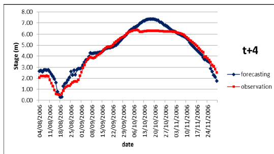
Fig. 30 Forecasting result of C.35 at time t+4
