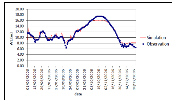
Fig. 12 Calibration result at Chao-Phraya dam station (C.13)
