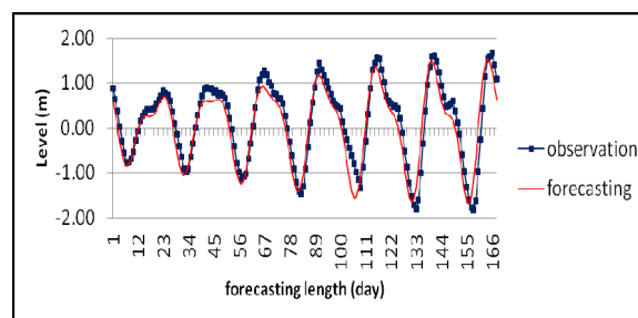
Fig. 15 Results of tidal level forecasting
