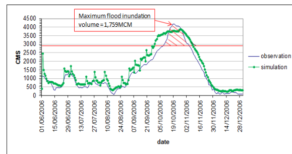
Fig. 33 Observed discharge at C.13
