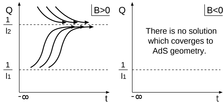
Fig. 5. Classical solutions Q(t) for A < 0 .
