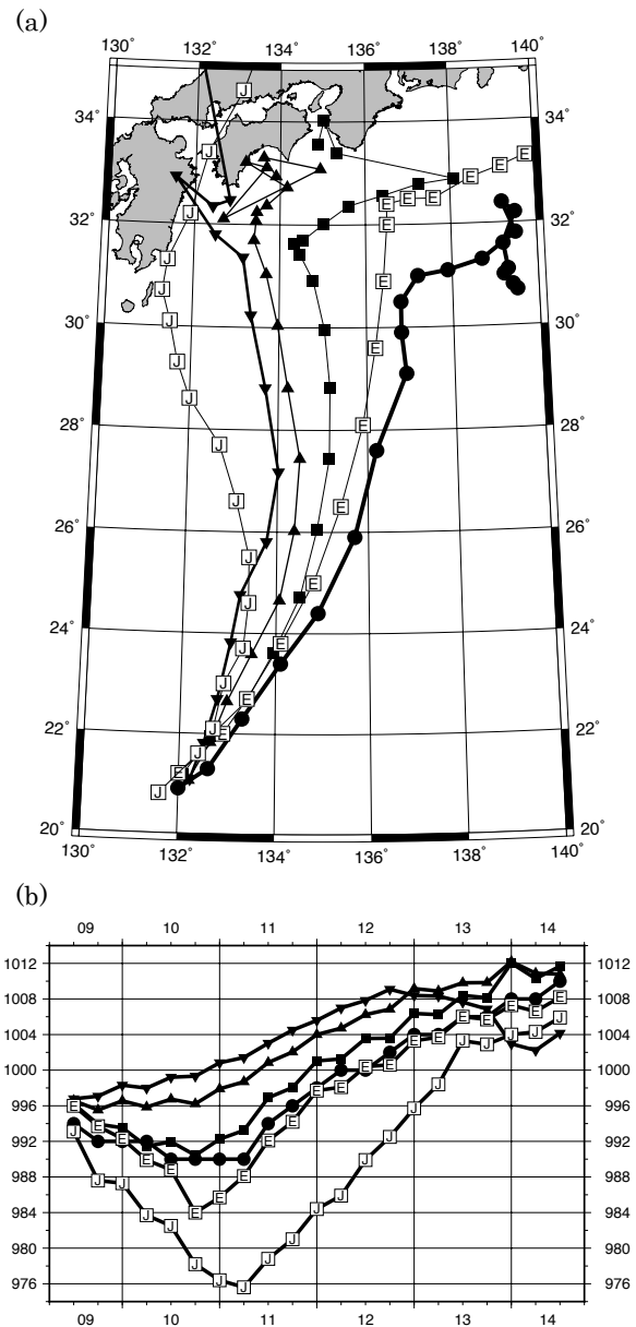
Fig. 2 (a) Track and (b) central pressure of Yagi 2013 in the RSMC Tokyo best track data, operational forecasts by JMA ( \square ) and by ECMWF ( \square ) and in forecast experiments using OpenIFS TL159 ( \blacktriangledown ), TL255 ( \blacktriangle ), TL511 ( \blacksquare ) L60 initialized with the operational ECMWF analysis at 12 UTC, 9 June 2013.
