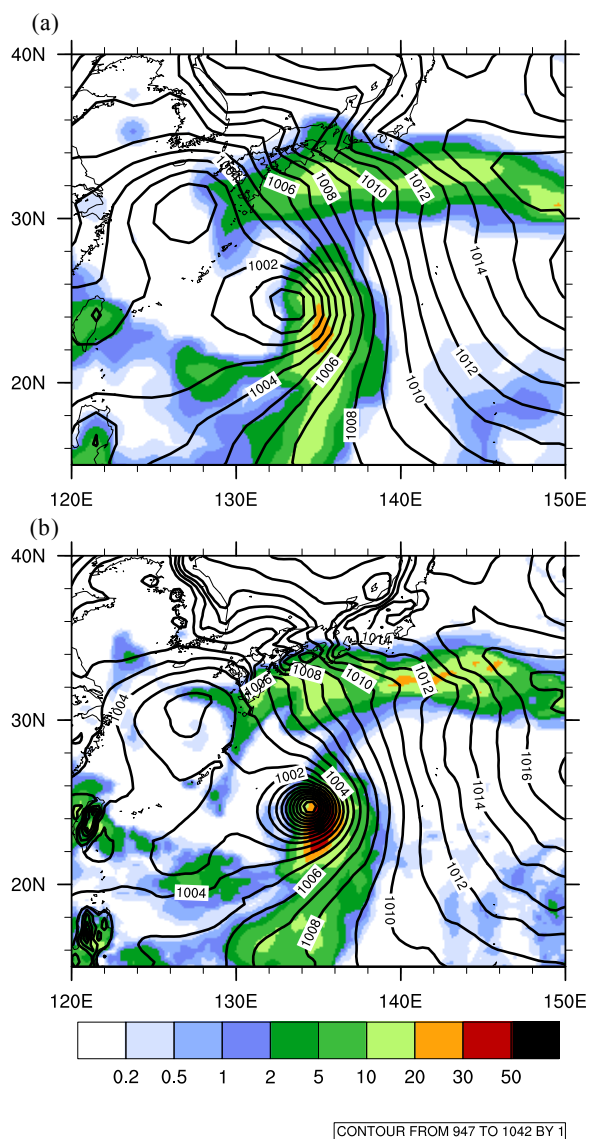
Fig. 3 24-hr forecast of sea-level pressure (contours) and 12-hr accumulated precipitation (mm, colour shades) with (a) TL159 and (b) TL511 resolution.
