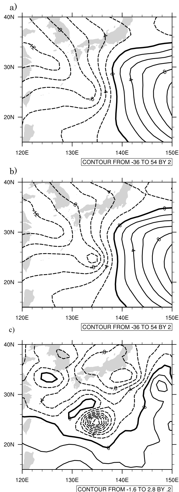
As in Fig. 3 but for 700-hPa stream function. The difference (TL511-TL159) is shown in (c).
