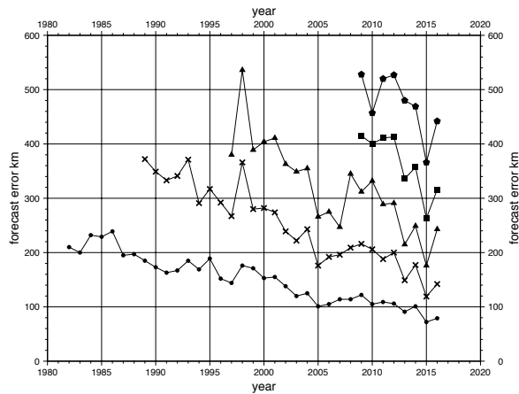
Fig. 1 Annual average of the forecast error for typhoon tracks by JMA. The 24, 48, 72, 96 and 120 (Japan Meteorological Agency, 2017)
