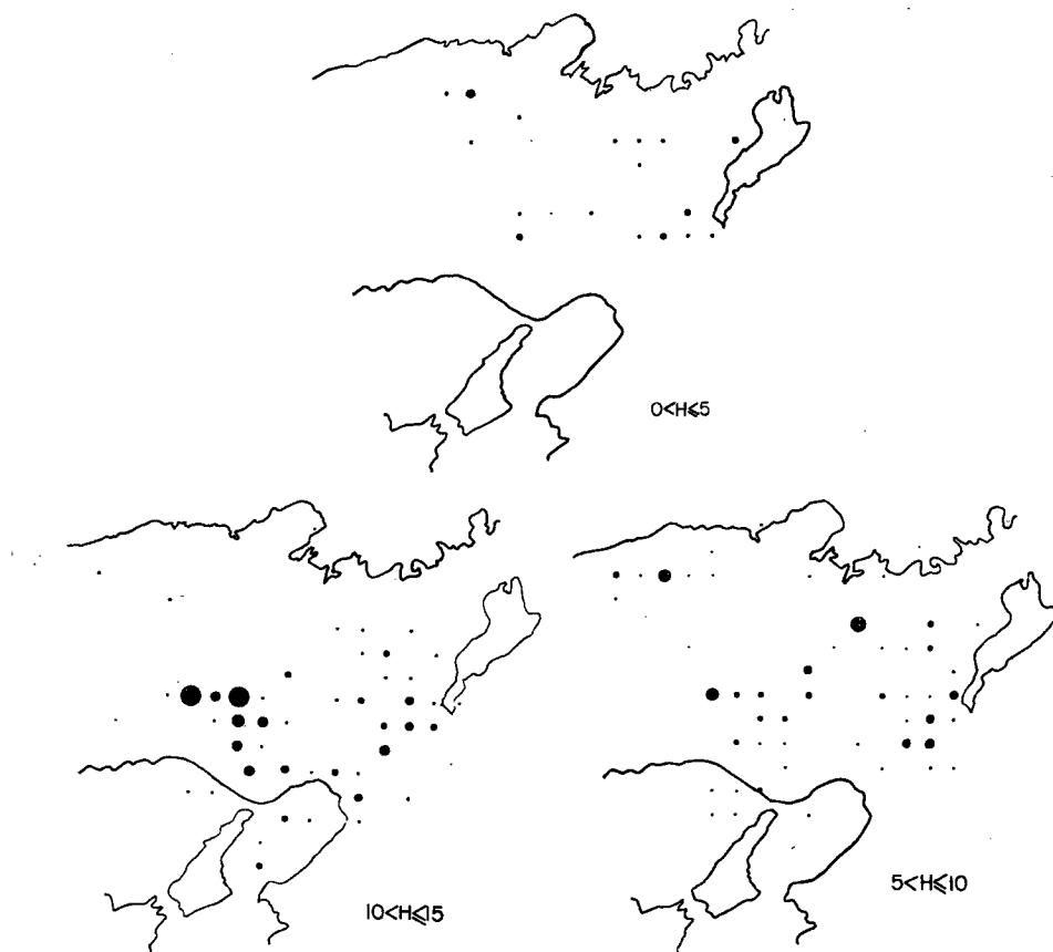
Fig. 3 Distribution of focal depth. Diameter of each circle is proportional to number of earthquakes generated in each mesh of 10 km × 10 km.
