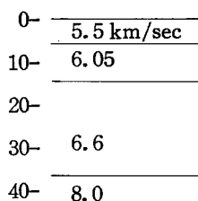
Fig. 1 Crustal structure assumed in the area concerned.
