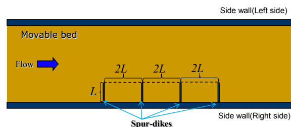
Fig. 2 Sketch of spur-dikes
