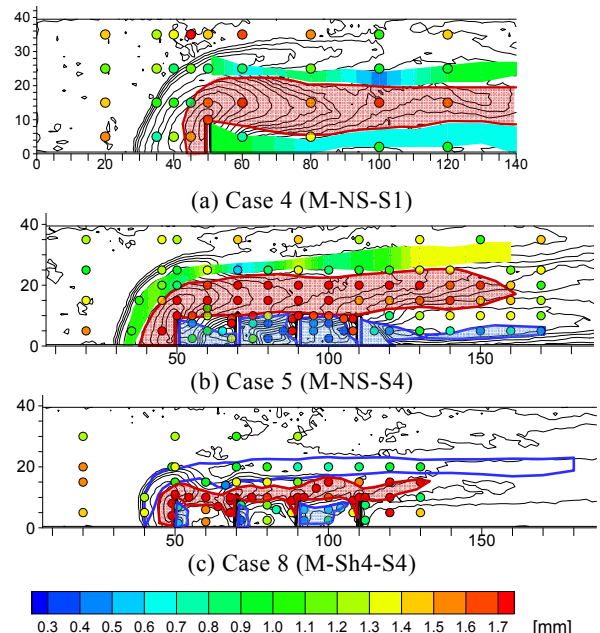
Fig. 11 Grain size distribution D_m ; (a) Case 4, (b) Case 5 and (c) Case 8 (circles: sampling points; belts: fine sediment belts; lines: bed contours)
