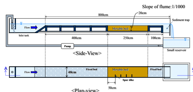
Fig. 1 Sketch of the experimental flume
