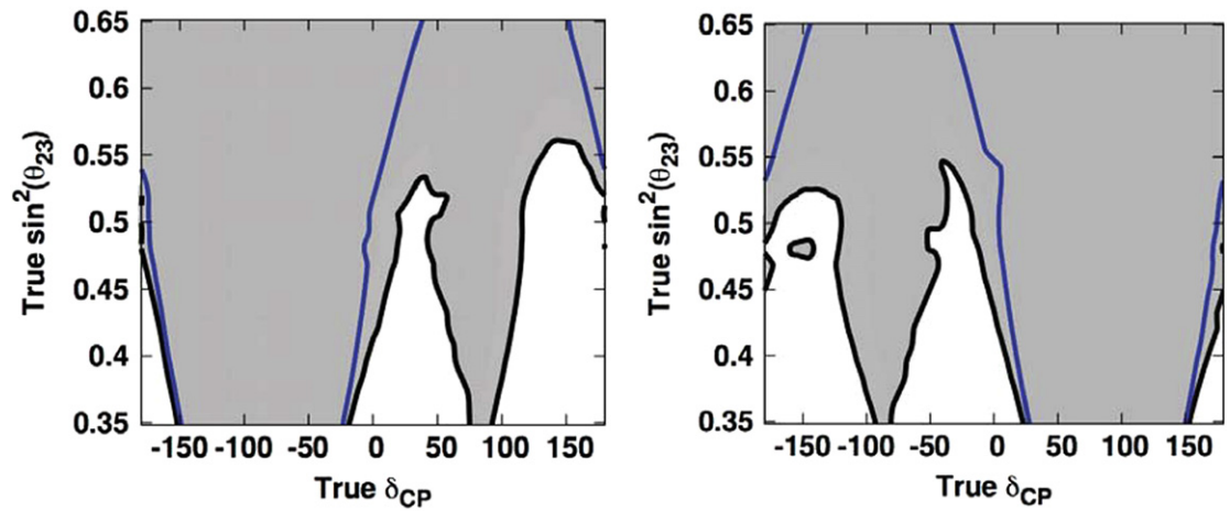
Figure 36. The regions where the wrong mass hierarchy is expected to be rejected at 90% C.L. by the NOvA measurement (blue line) and the NOvA + T2K measurements (black shaded regions) [53]. (Left) The true hierarchy is normal and (right) it is inverted. The T2K POT are assumed to be 3.9 \times 10^{21} POT for the neutrino beam mode and 3.9 \times 10^{21} for the anti-neutrino. The NOvA POT ( 3.6 \times 10^{21} ) are also assumed to be distributed to the neutrino beam mode and the anti-neutrino equally.
