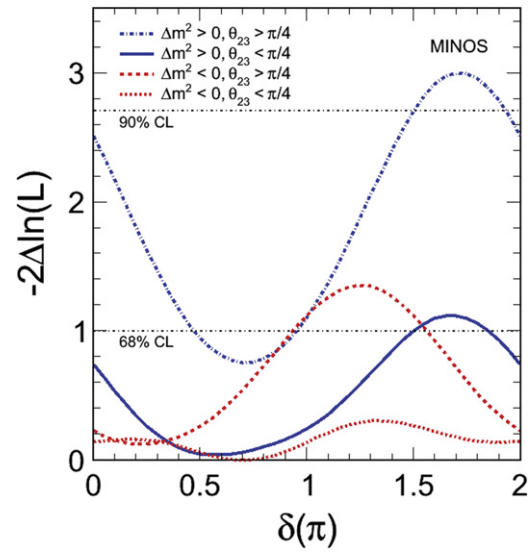
Figure 10. Variation of likelihood (compared to best fits) with \delta_{CP} , plotted as -2\Delta \ln(L) , for the observed \nu_e appearance in MINOS, shown for varying combinations of other oscillation parameters. Values above the horizontal dashed lines are disfavored at either 68% or 90% C. L.
