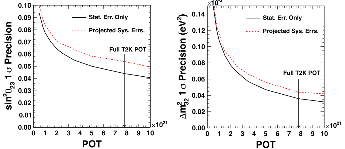
Figure 34. T2K expected sensitivity to \sin^2 \theta_{23} and |\Delta m_{32}^2| as a function of POT for the normal mass hierarchy [53]. The solid lines are without systematic error and the dashed one with the systematic error from the T2K 2012 analysis. POT are assumed to be 3.9 \times 10^{21} POT for the neutrino beam mode and 3.9 \times 10^{21} for the anti-neutrino.
