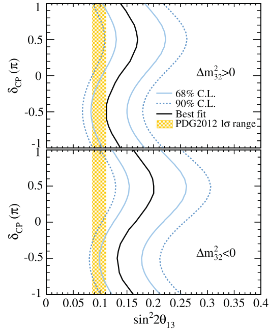
Figure 12. The allowed regions for \sin^2 2\theta_{13} as a function of \delta_{CP} for the normal mass hierarchy case (top) and the inverted one (bottom) from [3]. The value of \theta_{13} from reactor experiments in PDG2012 is shown as the shaded region.
