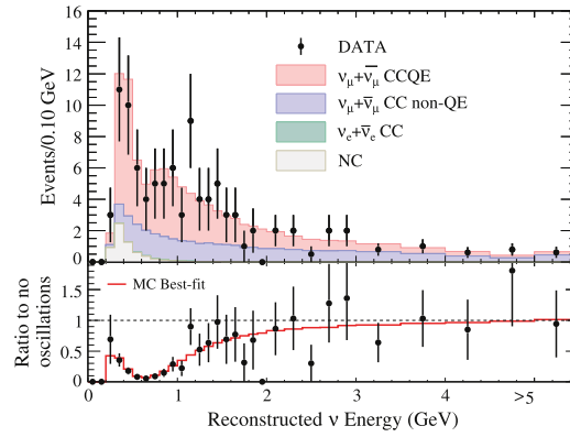
Figure 14. The neutrino energy spectrum for single-ring muon events in [2]. (Top) The observed and expected spectra with the event categories in the simulation. (Bottom) The ratio of the observed spectrum to the no-oscillation hypothesis with the best-fit case.
