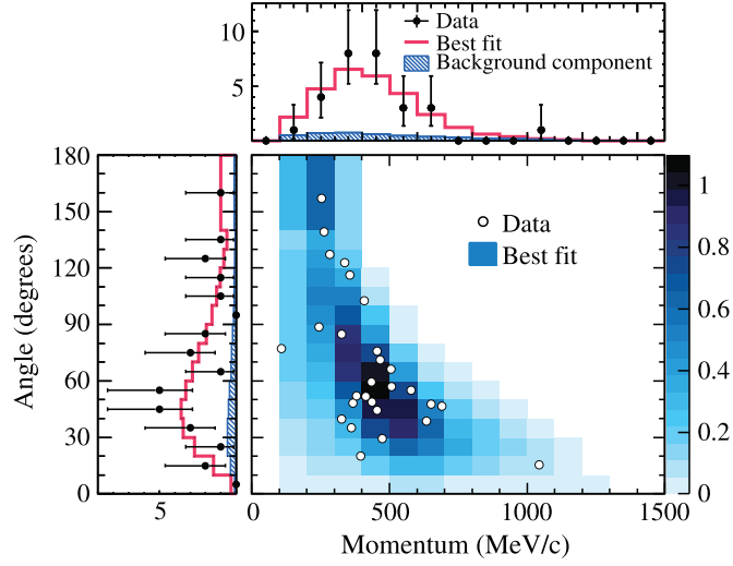
Figure 11. The T2K electron momentum versus angle distribution for 28 single-ring electron events, together with the MC expectation in [3]. The best fit value of \sin^2 2\theta_{13} = 0.140 in the normal hierarchy case is used for the expectation.
