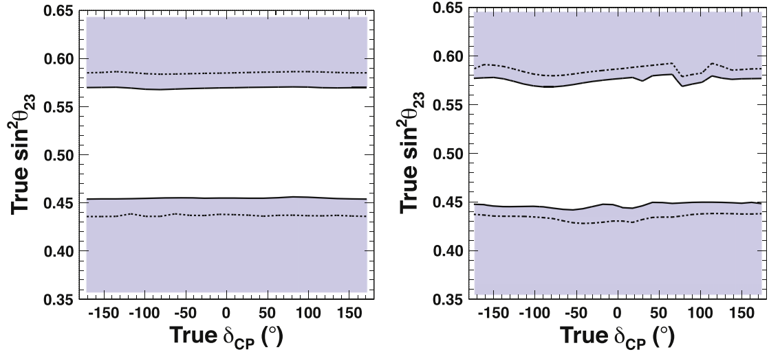
Figure 35. (Left) The shaded region is where T2K has more than a 90% C.L. sensitivity to reject maximal mixing [53]. (Right) The shaded region is where T2K has more than a 90% C.L. sensitivity to reject one of the octants of \theta_{23} [53]. The mass hierarchy is considered unknown in the normal mass hierarchy case. The shaded region is calculated assuming no systematic errors (statistical error only), and the dashed contours show the sensitivity including the systematic errors. POT are assumed to be 3.9 \times 10^{21} POT for the neutrino beam mode and 3.9 \times 10^{21} for the anti-neutrino.
