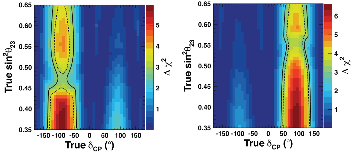
Figure 33. T2K expected \chi^2 difference between the true point ( \delta_{\text{CP}}, \sin^2 \theta_{23} ) and the point \delta_{\text{CP}} = 0 [53]. The map of \chi^2 difference shown in color is calculated assuming no systematic errors. The solid contours show the 90% C.L. sensitivity with statistical error only, while the dashed contours include the 2012 T2K systematic error. (Left) The contour in the case of normal mass hierarchy, and (right) in the case of Inverted mass hierarchy. POT are assumed to be equally distributed to the neutrino beam mode ( 3.9 \times 10^{21} POT) and the anti-neutrino ( 3.9 \times 10^{21} POT).
