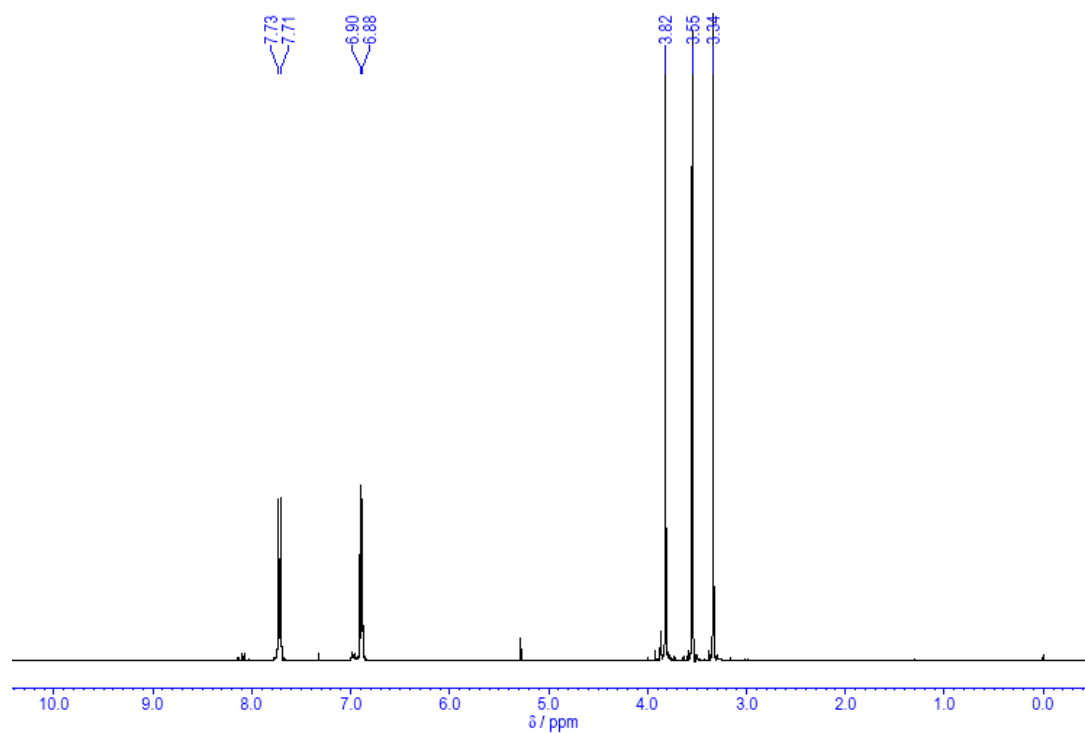
Figure S3. 1 H NMR spectrum of 1b in CDCl 3 .
