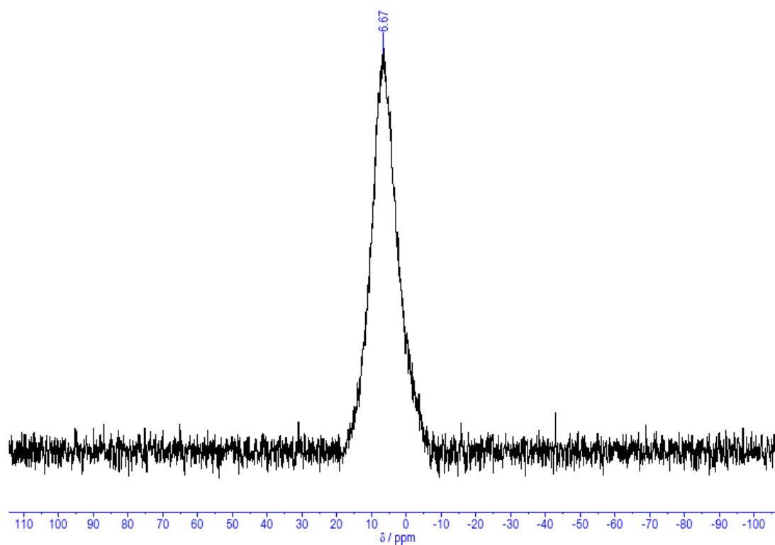
Figure S16. 11 B NMR spectrum of para -BMeO in CDCl 3 .
