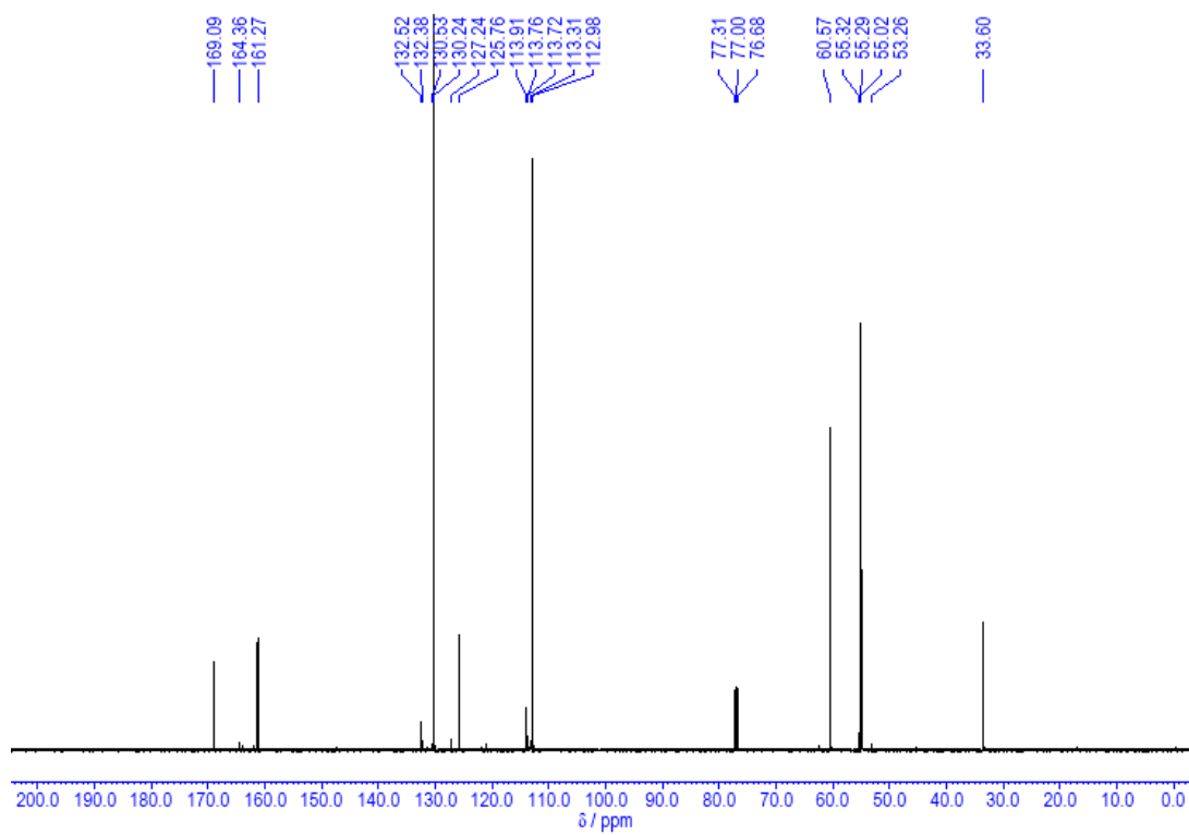
Figure S4. 13 C NMR spectrum of 1b in CDCl 3 .
