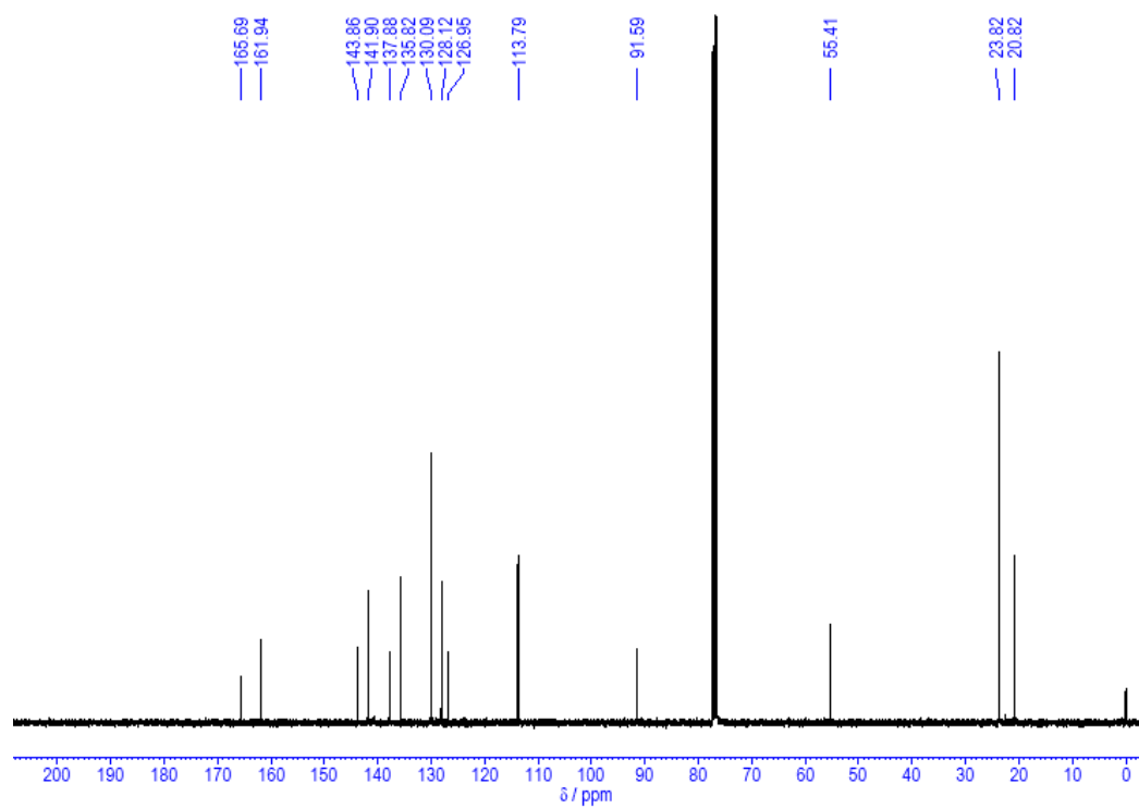
Figure S15. 13 C NMR spectrum of para -BMeO in CDCl 3 .
