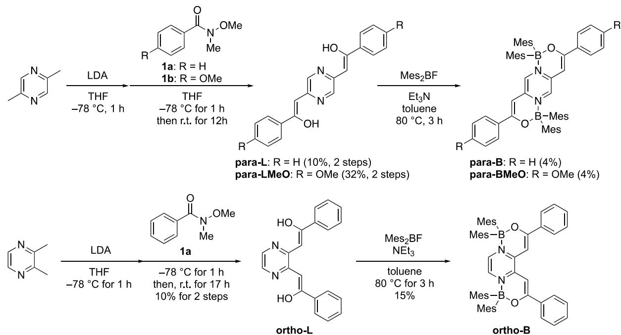
Scheme 1. Synthetic scheme of pyrazine-based boron complexes
