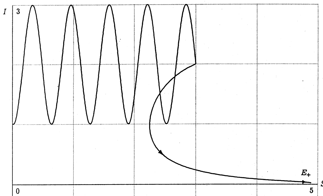
Figure 2. The graph of the trajectory of (3.2) with \alpha = 0.49 , h = 30 and the initial function \varphi_1(\theta) = 0.1\theta + 3 and \varphi_2(\theta_2) = 2 - \sin(\theta) for \theta \in [-h, 0] .
