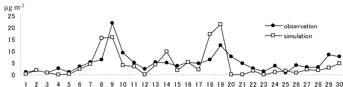
Fig. 8 : Comparison of daily sulfate concentrations simulated with observed at Haplo in April 2001.
