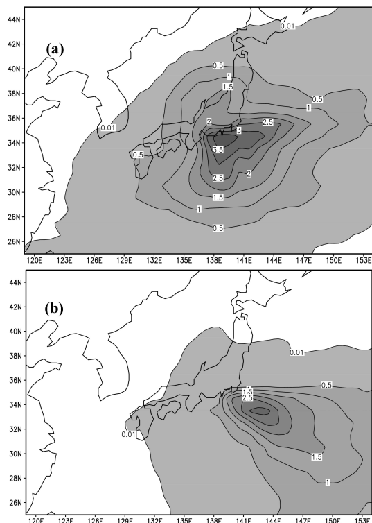
Fig. 13 : Seasonal variations of the volcanic sulfate concentration within PBL in (a) October 2000 and (b) January 2001.
