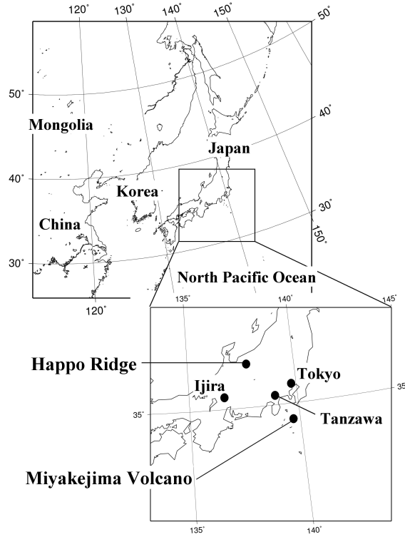
Fig. 3 : A decription of Far East Asia, Haplo Ridge, Miyakejima Volcano and other locations mentioned in this paper.
