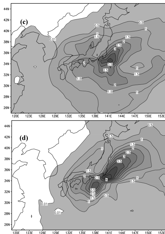
Same as the left figure but in (c) April 2001 and (d) July 2001.
