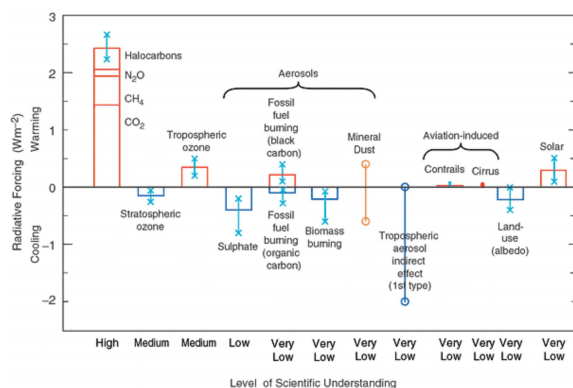
Fig. 1 : Global, annual-mean radiative forcings ( \text{Wm}^{-2} ) due to a number of agents for the period from pre-industrial (1750) to present (late 1990s; about 2000) same as fig. 9 in IPCC report, Climate Change 2001 : Working Group 1.
