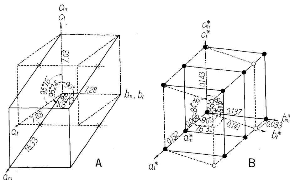
Fig. 1. Relationship between the unit cells of parawollastonite (solid lines) and wollastonite (broken lines). A. Direct cells, cross marks denote the intersecting points of edges of the two cells. B. Reciprocal cells, there are two reciprocal cells of parawollastonite.
