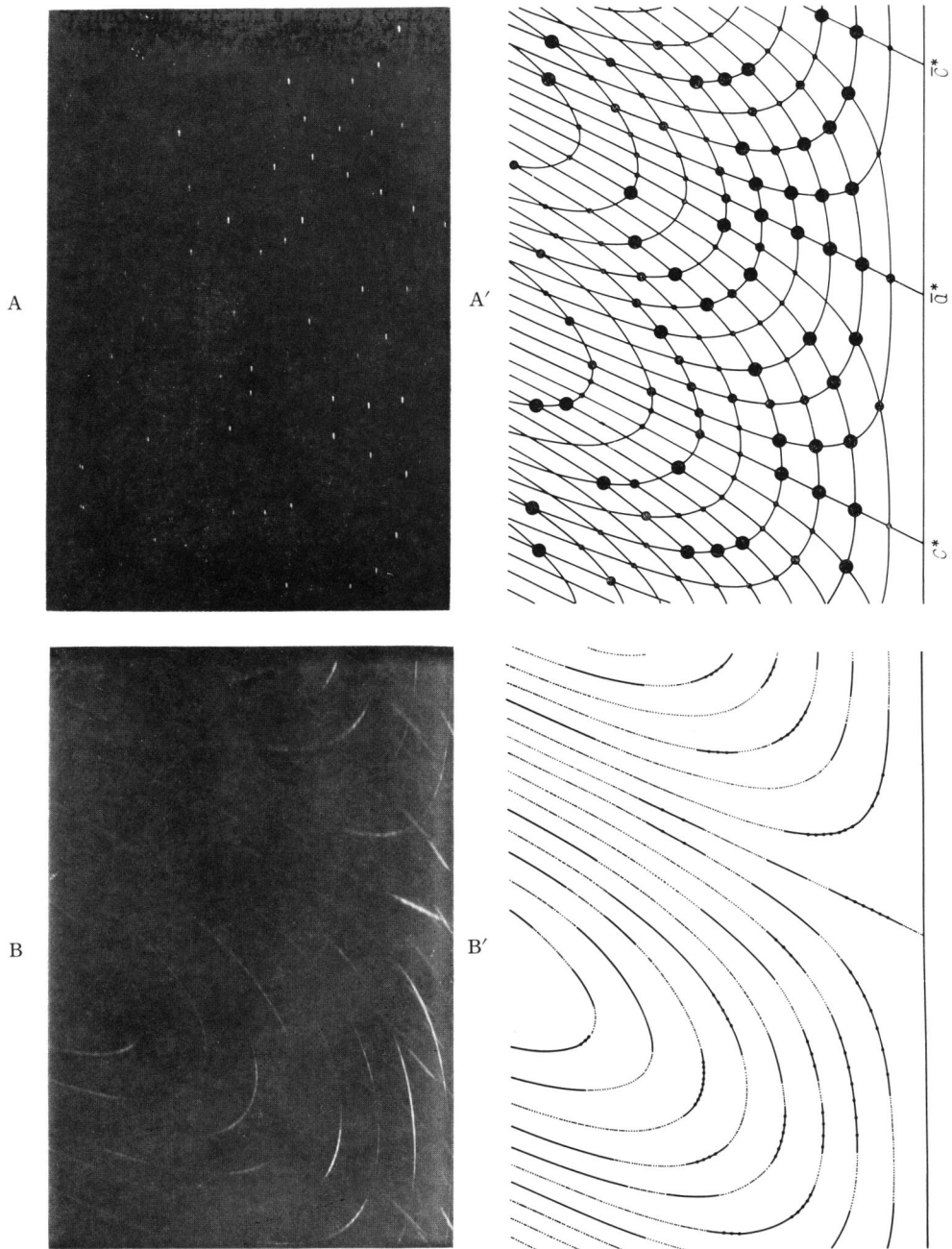
Fig. 5. Equi-inclination Weissenberg photographs of a specimen from Baba. A, A'. The zero layer. B, B'. The 1st layer.
