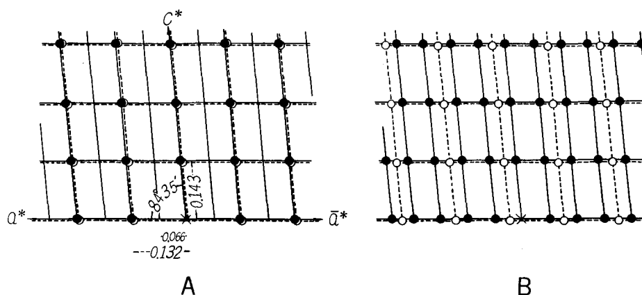
Fig. 2. Reflexions which should appear in the equi-inclination Weissenberg photographs about b -axis when the photographs are taken with parawollastonite and wollastonite. Solid circles denote reflexions for parawollastonite and open circles reflexions for wollastonite. A. The zero layer. B. The 1st layer.
