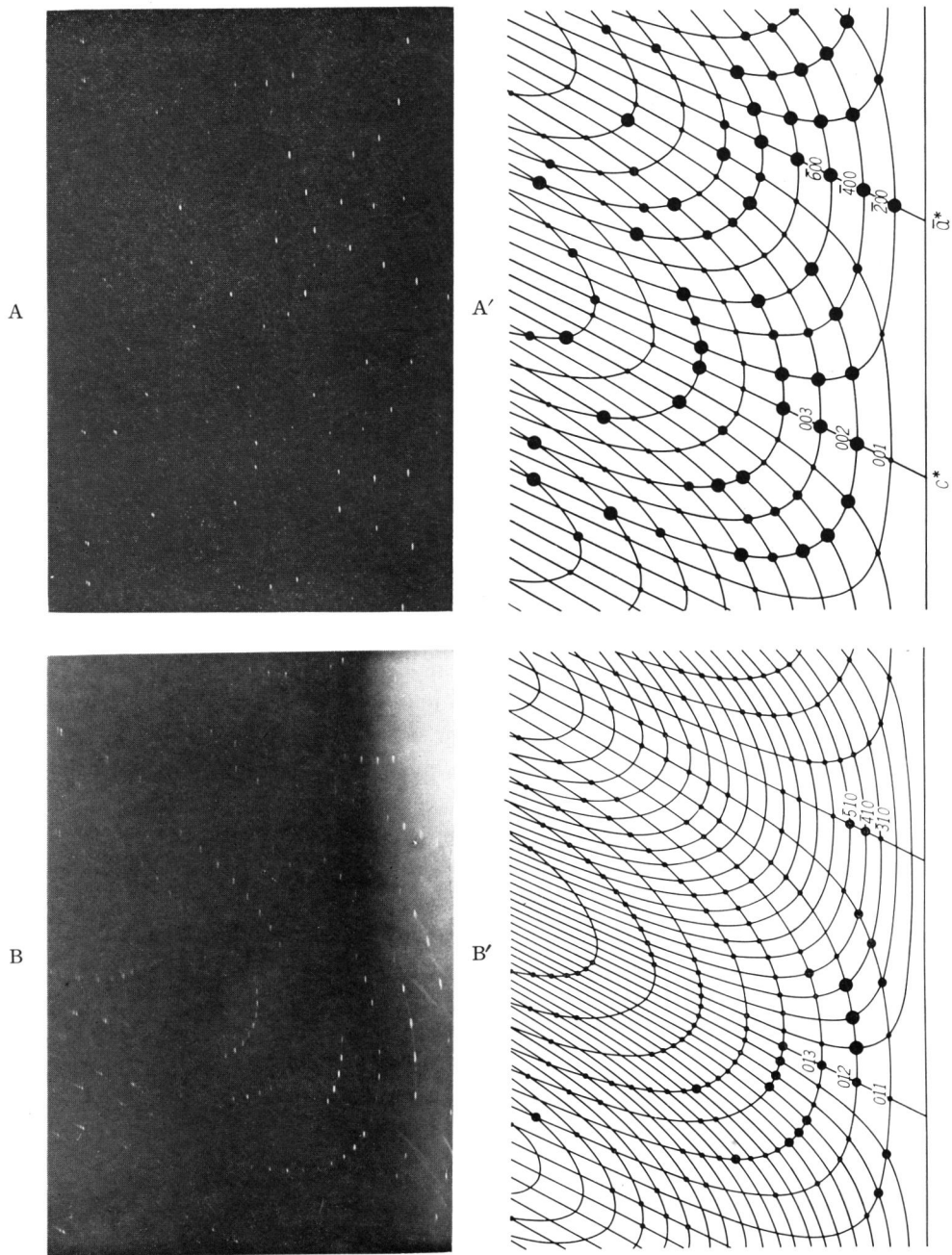
Fig. 4. Equi-inclination Weissenberg photographs of a specimen from Azukuji. A, A'. The zero layer. B, B'. The 1st layer.
