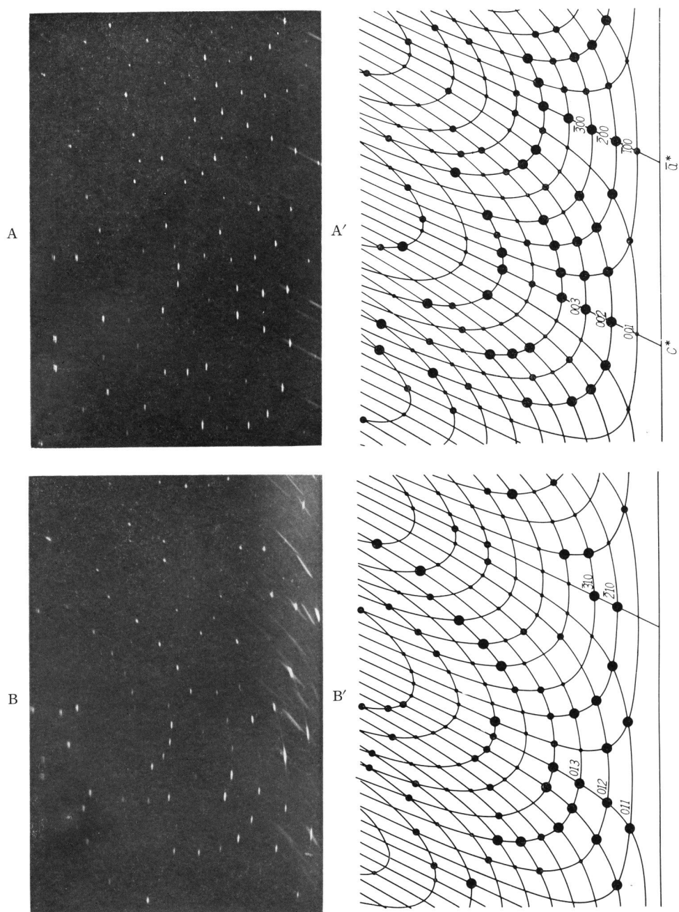
Fig. 3. Equi-inclination Weissenberg photographs of a specimen from Aotani. A, A'. The zero layer. B, B'. The 1st layer.
