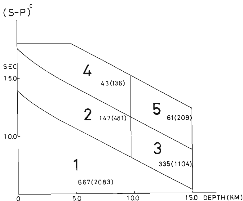
Fig. 23. Classification for studying the Poisson's ratios. The large numerals in each block are the classification numbers. The small numerals in and out of parentheses are the numbers of the S - P data and of the earthquakes respectively used in the relevant blocks.
