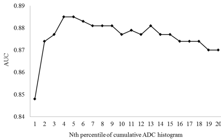
Fig. 1. Measurements of areas under ROC curve at multiple Nth percentiles (from the first to 20th percentile) of cumulative ADC histogram. The 4th and 5th percentiles have the largest AUC value.
