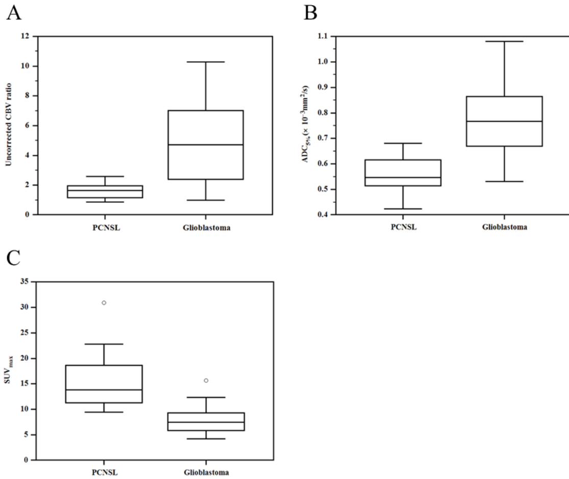
Fig. 2. Box-and-whisker plots of uncorrected CBV ratio (A), ADC_{5\%} (B), and SUV_{\max} (C) for PCNSL and glioblastoma. The central boxes represent the values from the lower to upper quartile (25th to 75th percentile). The middle lines represent the median. The vertical lines on each box indicate the range of data distribution. Values outside of 1.5 times of the interquartile range are presented with open circles.
