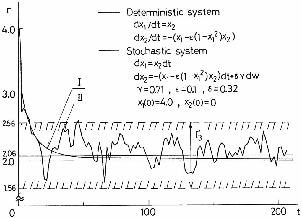
Fig.4.6 Sample Behavior of the System given by Eq.(4.39) (The Case of I'_3 = [1.56, 2.56] )
