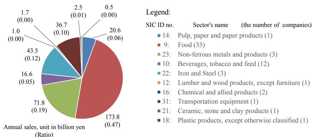
Fig. 2 Annual sales in 2010 of the industrial sectors of Hachinohe city in the inundation area due to the 2011 Tohoku tsunami
