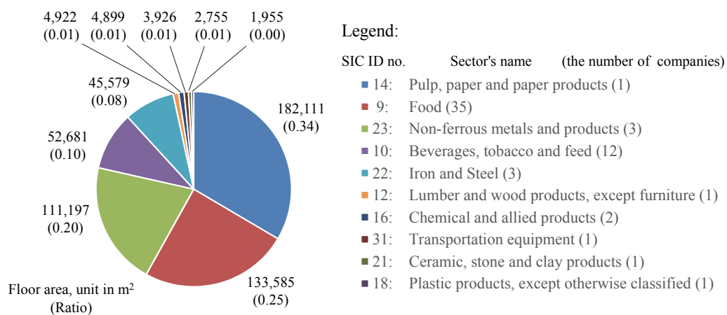
Fig. 1 Floor area of the 60 companies of the 10 industrial sectors of Hachinohe city in the inundation area due to the 2011 Tohoku tsunami
