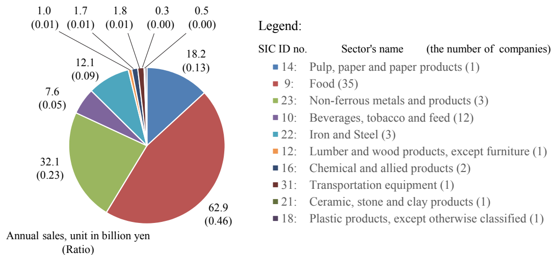
Fig. B.1 Annual sales in 2010 of the industrial sectors of Hachinohe city in the inundation area due to the 2011 Tohoku tsunami, estimated with "simple" method
