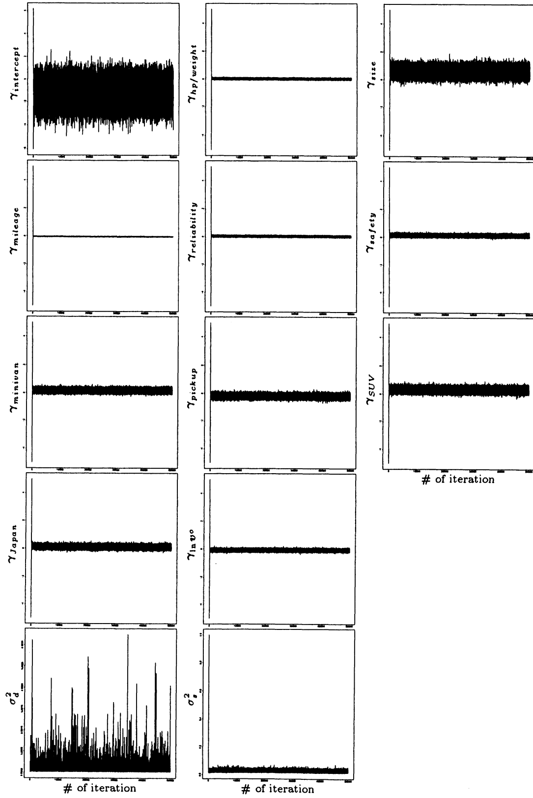
Figure 3: Time series plots for \gamma , \sigma_d^2 and \sigma_s^2 .
