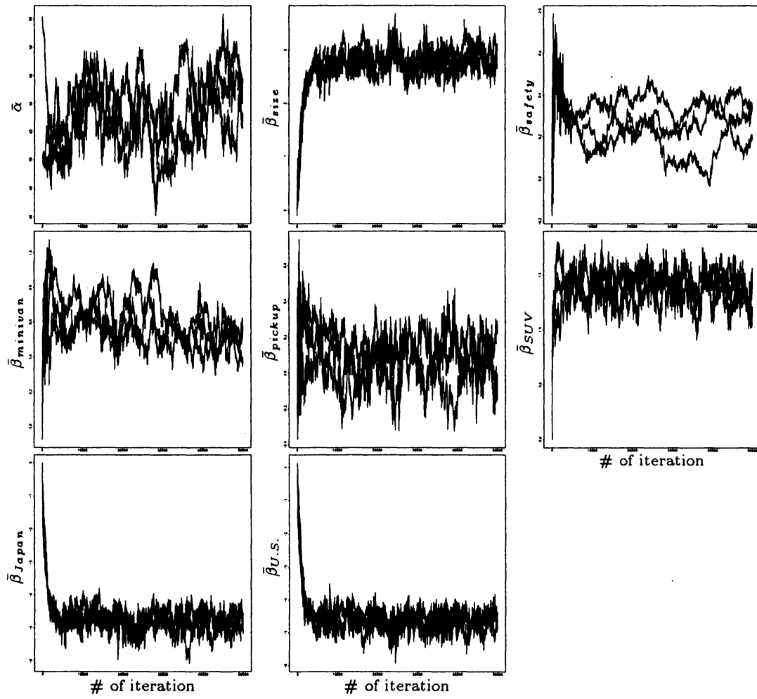
Figure 1: Time series plots for \bar{\theta} .
