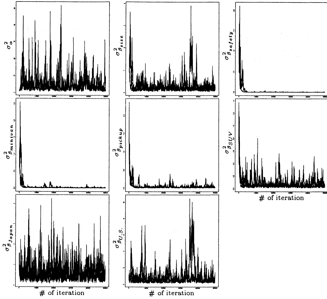
Figure 2: Time series plots for the diagonal components of \Sigma_{\theta} .
