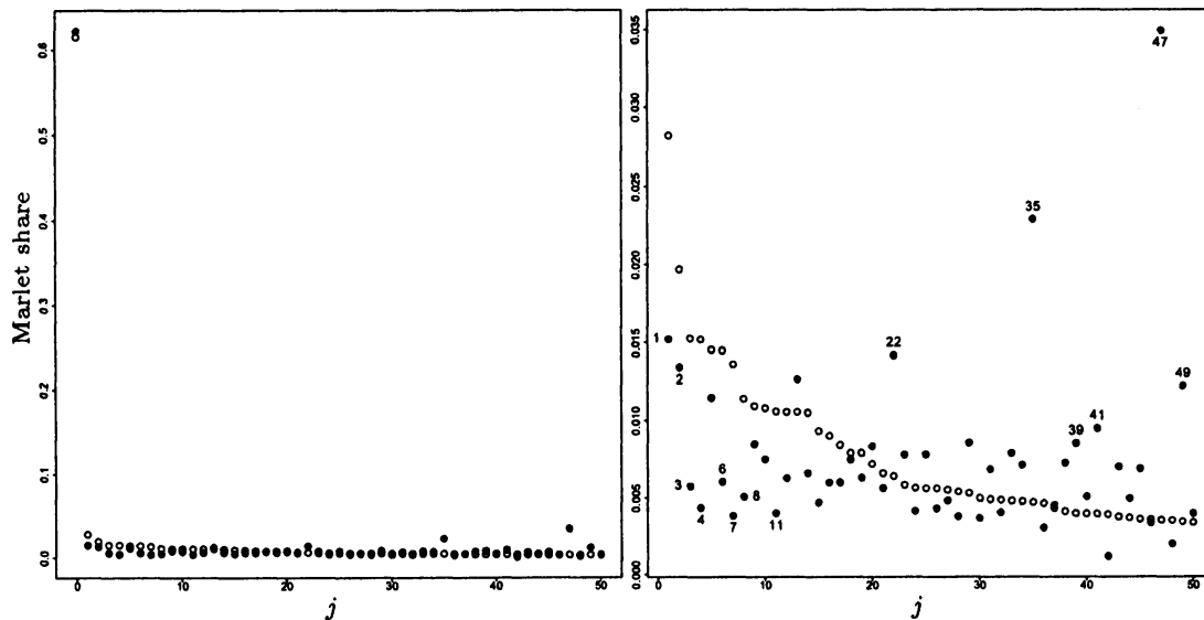
Figure 4: Predicted and observed market shares for the top 50 in sales of the 1996 models.
