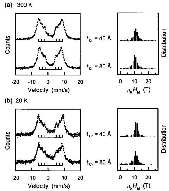
FIG. 2. ^{119}\text{Sn} Mössbauer spectra for [\text{Cr}(t_{Cr})/\text{Sn}(2 \text{ Å})] multilayers ( t_{Cr} = 40 and 80 \text{ Å} ) at (a) 300 K and (b) 20 K. The distribution of the magnetic hyperfine field obtained from the fitting of the spectra is shown on the right.
