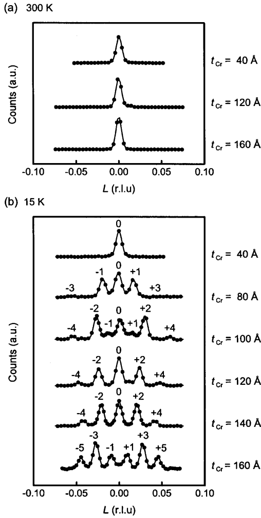
FIG. 1. Neutron diffraction patterns around Cr(010) along the L direction for [\text{Cr}(t_{Cr})/\text{Sn}(2 \text{ Å})] at (a) 300 K and (b) around 15 K. The peak positions for the patterns at 15 K are identified with a unit of \Delta \equiv a_{001}/(2\Lambda_{SL}) as L (r.l.u.) = \pm N\Delta ( N = 0, 1, 2, \dots ) (see the text).
