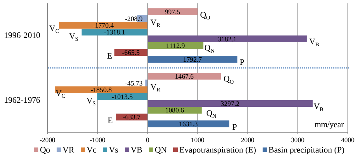
Figure 5-4 Annual average water balance components in the Kamo River Basin for the periods 1962-1976 and 1996-2010 (Minus value represents water going out from the basin)
