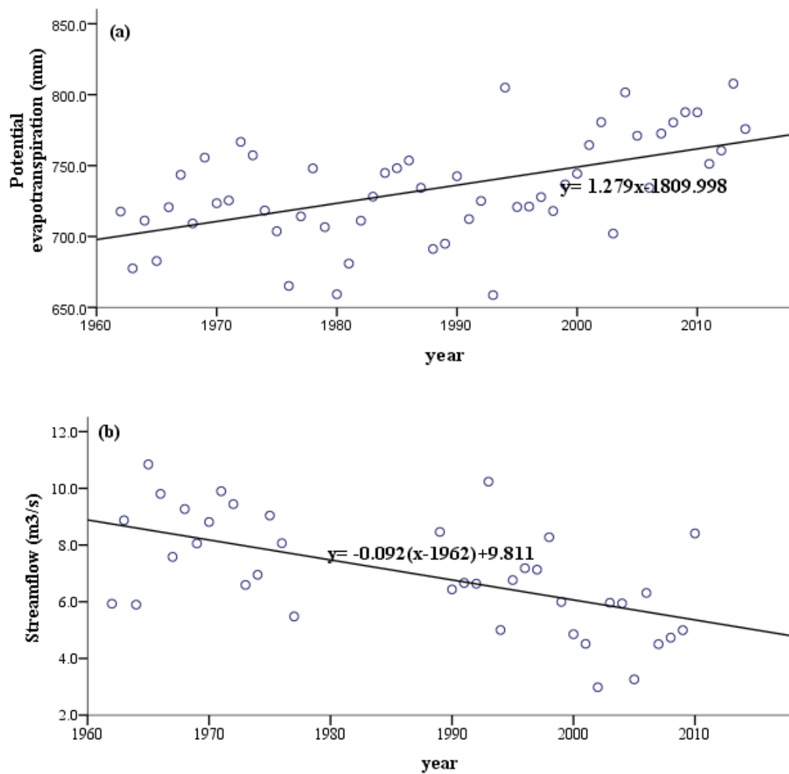
Figure 4-2 Time series of (a) potential evapotranspiration and (b) observed streamflow at Fukakusa station in the Kamo River basin
