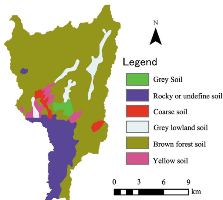
Figure 2-4 Soil type of KRB
