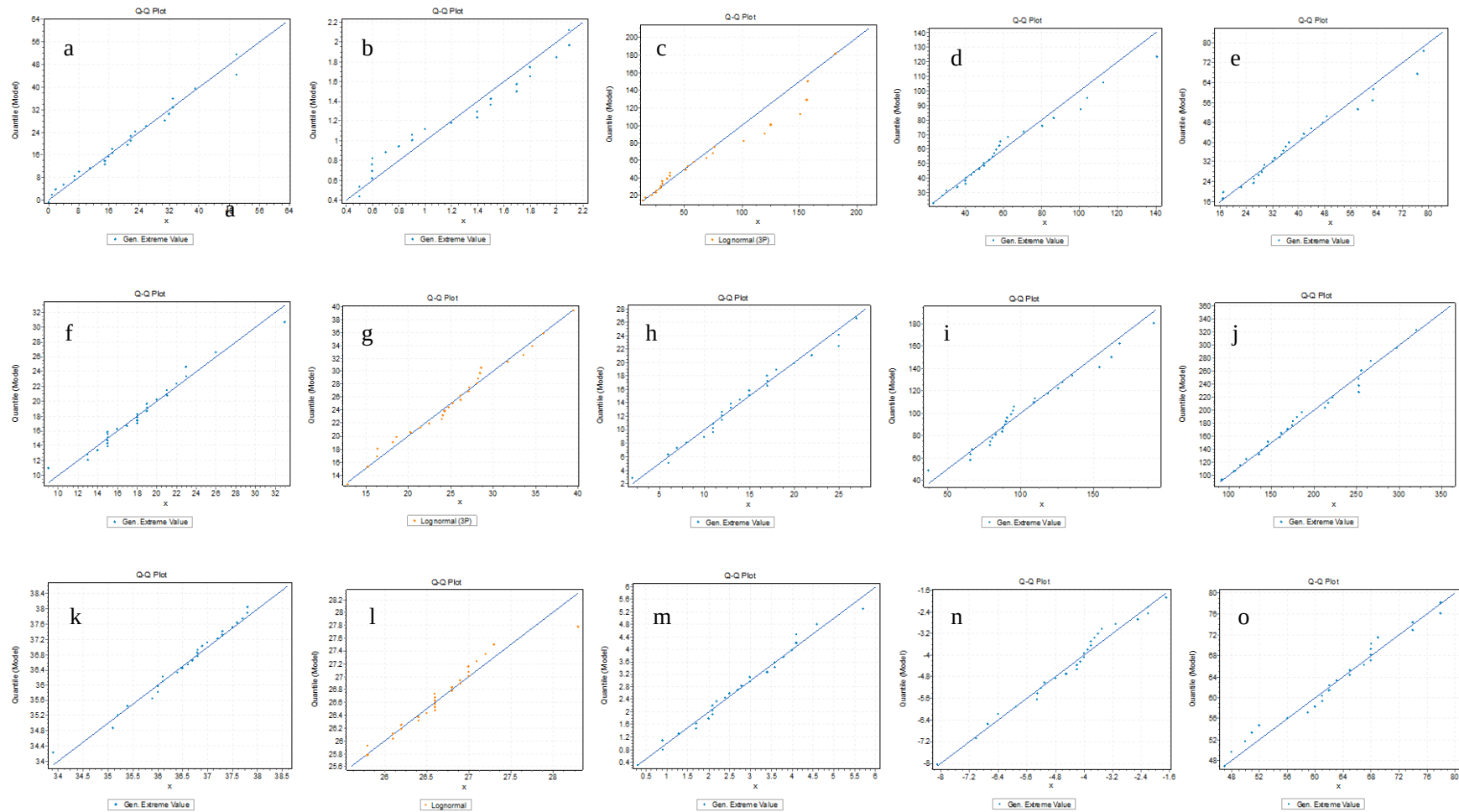
Figure 6-3 Quantile-Quantile (Q-Q) plots of extreme indices fitted for optimal distribution in the period 1962-1988: a) CDS, b) SN7day, c) SX1hour, d) SX1day, e) SX5day, f) CDD, g) RX1hour, h) R10mm, i) RX1day, j) RX5day, k) TXx, l) TNx, m) TXn, n) TNN, o) HT.
