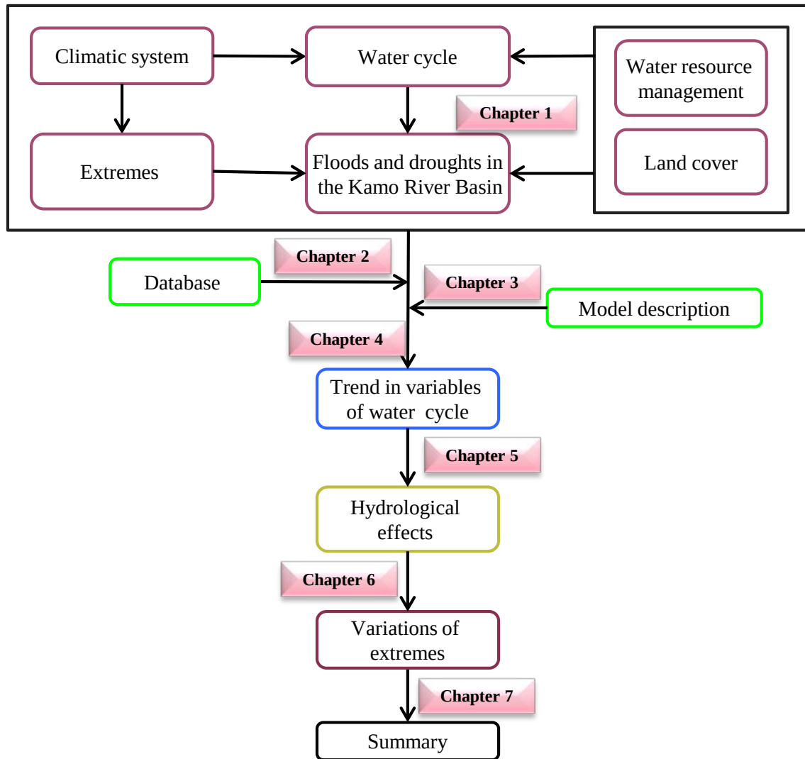
Figure 1-1 Framework of the thesis
