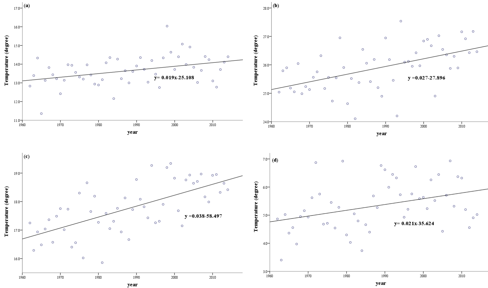
Figure 4-5 Time series of air temperature (a) spring, (b) summer, (c) autumn and (d) winter in the Kamo River basin
