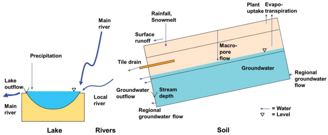
Figure 3-1 Schematic figure of one sub-basin of the HYPE model with one hydrological response unit (HRU, redrawn from Strömqvist et al., 2012)
