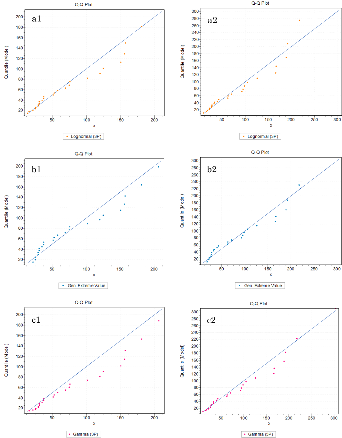
Figure 6-1 Quantile-Quantile (Q-Q) plots of SX1hour with different distributions in the period 1962-1988 and 1989-2014: a1) LN3 in the period 1962-1988; a2) LN3 in the period 1989-2014; b1) GEV in the period 1962-1988; b2) GEV in the period 1989-2014; c1) Gamma in the period 1962-1988; c2) Gamma in the period 1989-2014.
