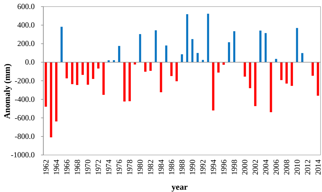
Figure 4-3 Time series of annual basin average precipitation anomalies in the Kamo River basin with respect to the average value from 1981 to 2010
