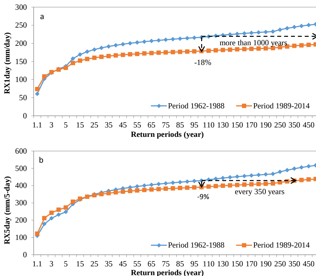
Figure 6-8 Annual inverse cumulative distribution functions of extreme precipitation indices: a) RX1day and b) RX5day
