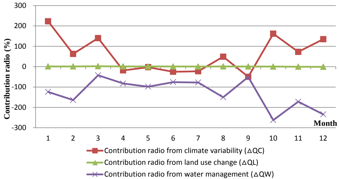
Figure 5-7 Contribution ratio of different factors to streamflow in the Kamo River basin for the periods 1962-1976 and 1996-2010 (Minus value represents water going out from the basin)
