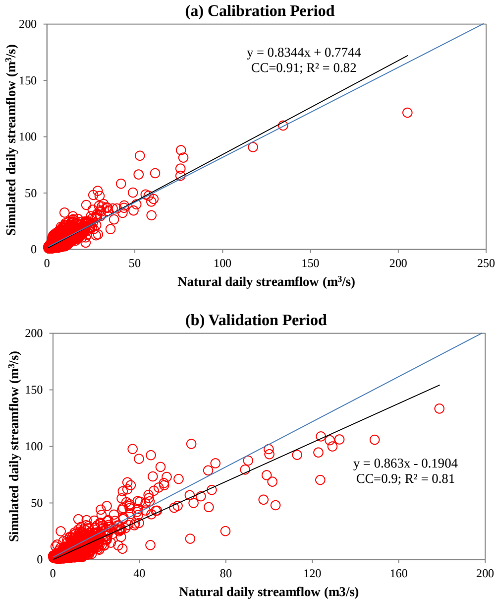
Figure 5-3 Correlation between daily simulated and natural streamflow in (a) calibration and (b) validation periods
