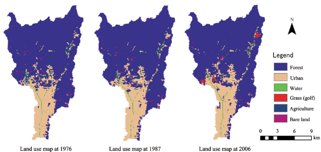
Figure 2-5 Land use types of the Kamo River basin
