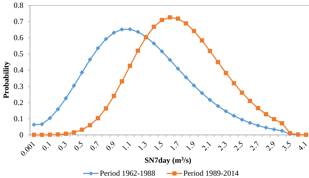
Figure 6-6 Annual probability distribution functions of SN7day index
