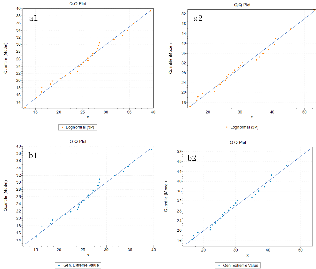
Figure 6-2 Quantile-Quantile (Q-Q) plots of RX1hour with different distributions in the period 1962-1988 and 1989-2014: a1) LN3 in the period 1962-1988; a2) LN3 in the period 1989-2014; b1) GEV in the period 1962-1988; b2) GEV in the period 1989-2014
