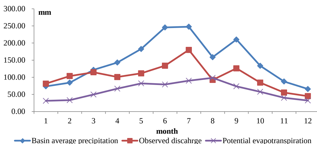
Figure 4-9 Average monthly hydro-climatic variables from 1962 to 2014 in millimeter in the Kamo River basin
