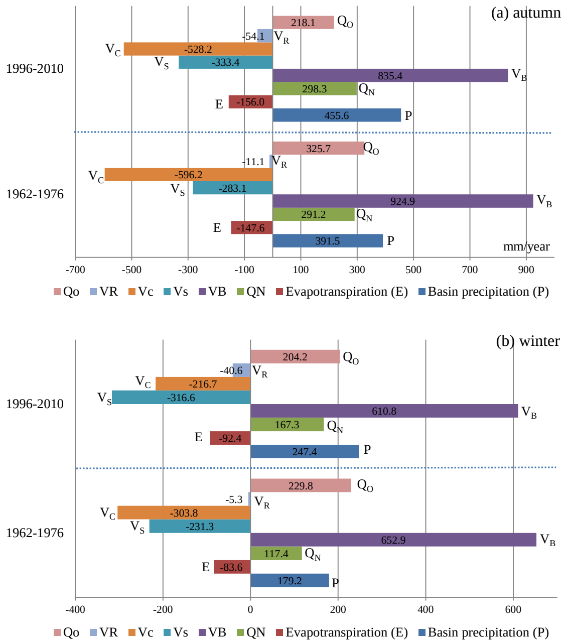
Figure 5-6 Seasonal average water balance components for the periods 1962-1976 and 1996-2010 (Minus value represents water going out from the basin) (a) autumn (b) winter
