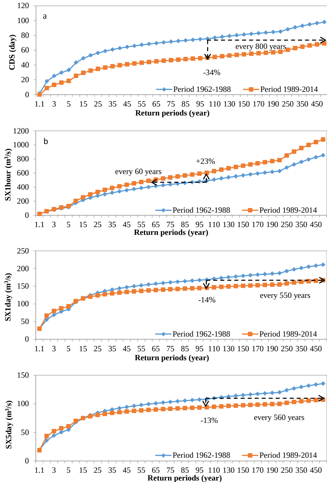
Figure 6-5 Annual inverse cumulative distribution functions of river discharge indices: a) CDS, b) SX1hour, c) SX1day, d) SX5day
