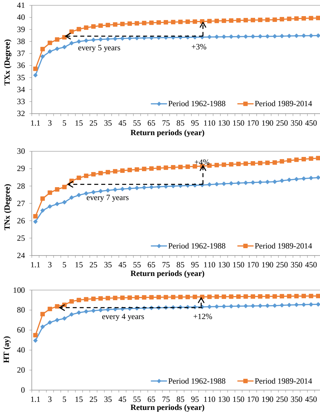
Figure 6-9 Annual inverse cumulative distribution functions of extreme temperature indices: a) TXx, b) TNx, c) HT
