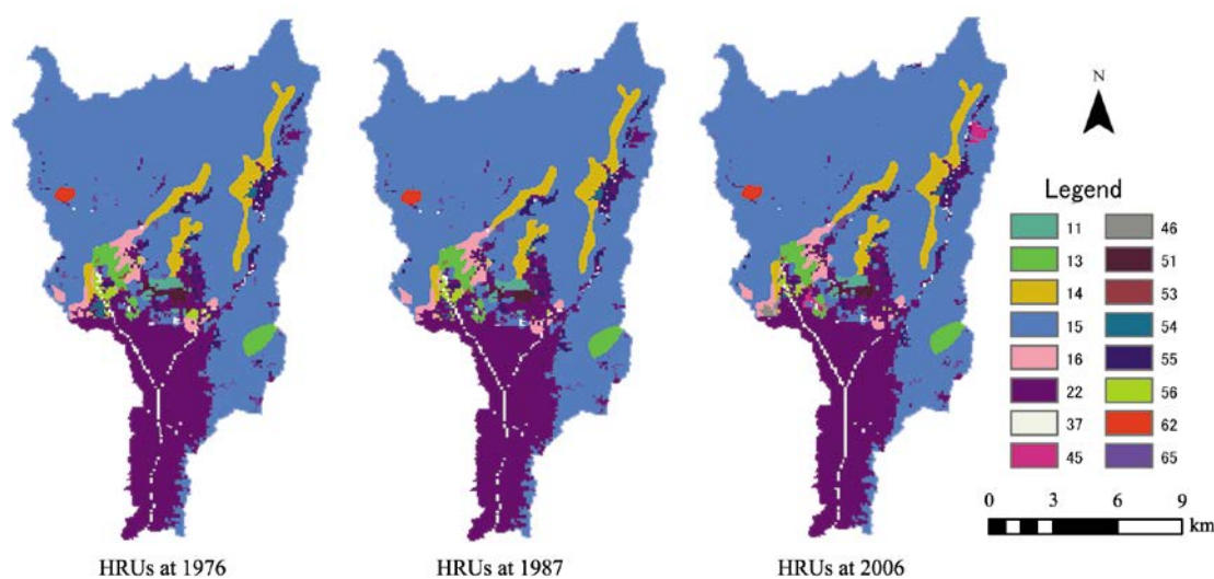
Figure 3-2 Hydrological response units (HRUs) at different periods in the Kamo River basin
