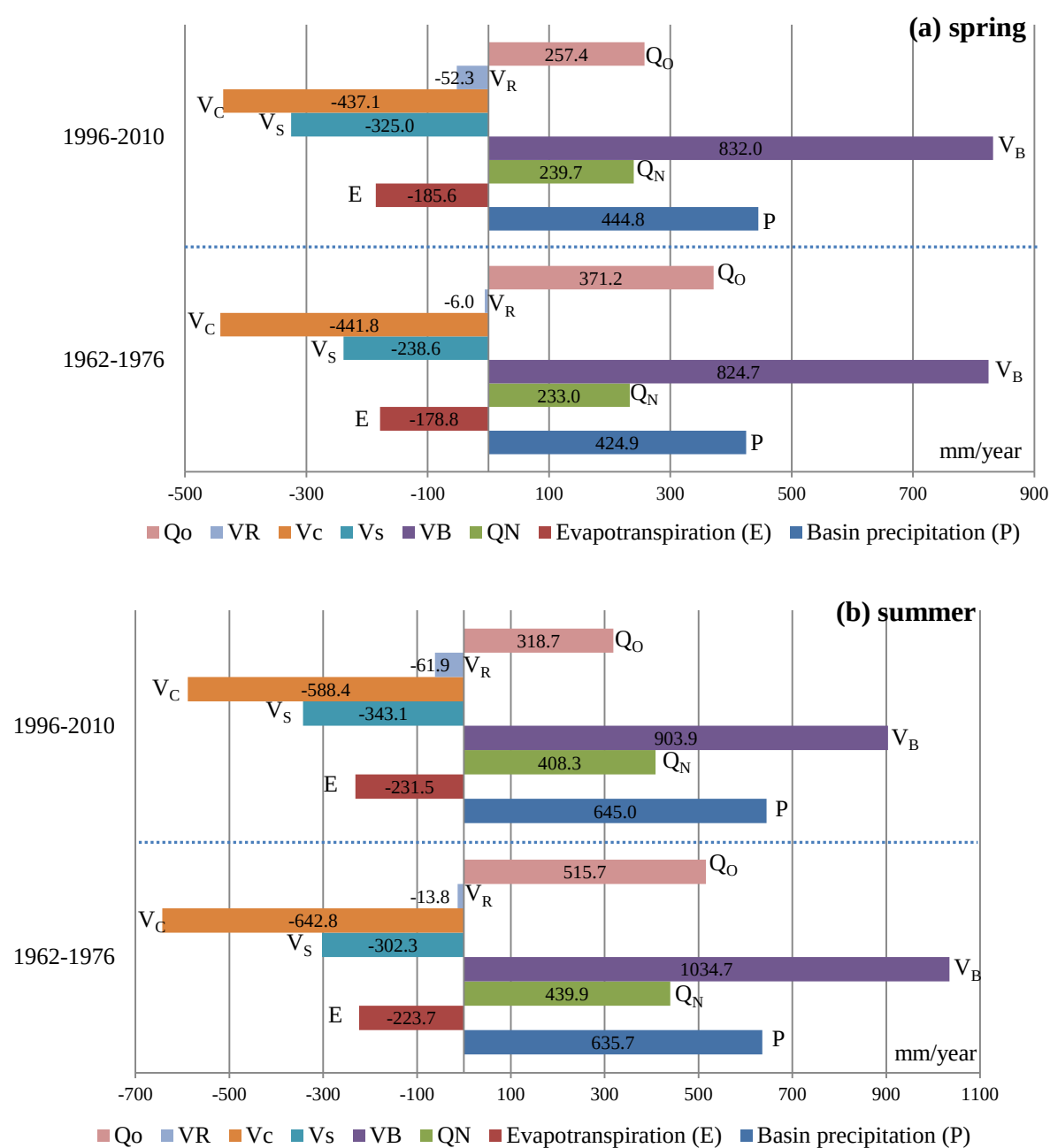
Figure 5-5 Seasonal average water balance components for the periods 1962-1976 and 1996-2010 (Minus value represents water going out from the basin) (a) spring (b) summer
