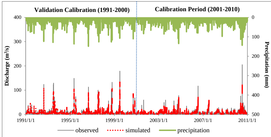
Figure 5-2 Comparison of simulated and natural daily streamflow at KRB outlet
