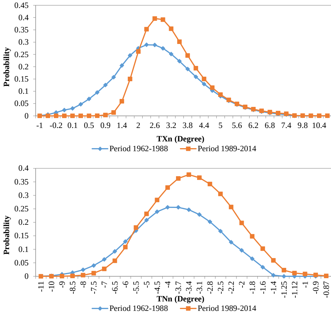
Figure 6-10 Annual probability distribution functions of TXn and TNn
