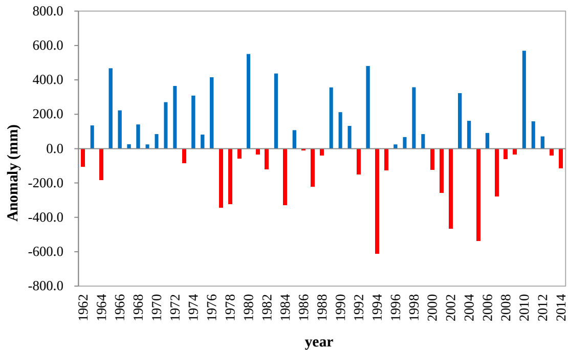
Figure 4-4 Time series of annual precipitation anomalies at Kyoto station in the Kamo River basin with respect to the average value from 1981 to 2010
