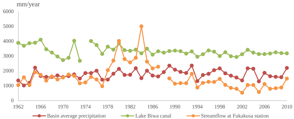
Figure 5-1 Annual statistics of observed data from 1962 to 2010
