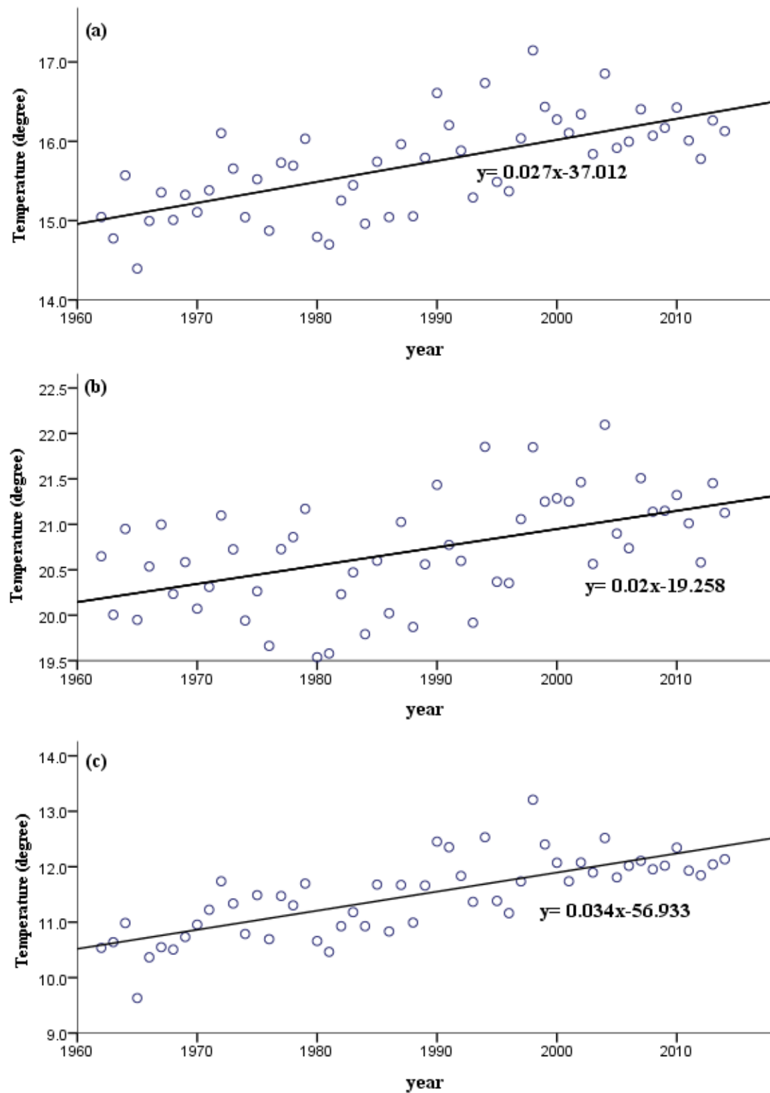
Figure 4-1 Time series of (a) air temperature, (b) maximum temperature and (c) minimum temperature in the Kamo River basin
