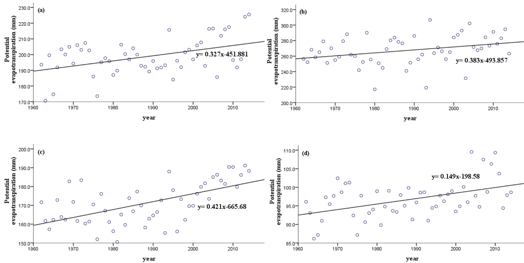
Figure 4-6 Time series of potential evapotranspiration (a) spring, (b) summer, (c) autumn and (d) winter in the Kamo River basin
