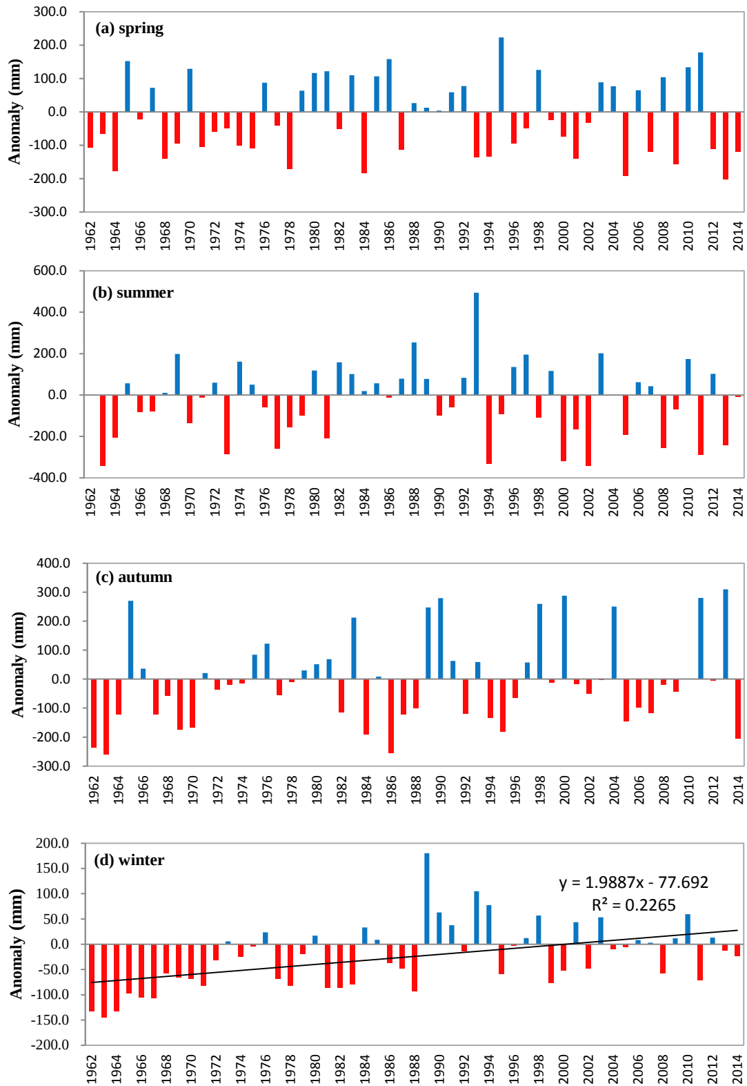
Figure 4-8 Time series of seasonal basin precipitation anomalies (a) spring, (b) summer, (c) autumn and (d) winter in the Kamo River basin with respect to the average value from 1981 to 2010
