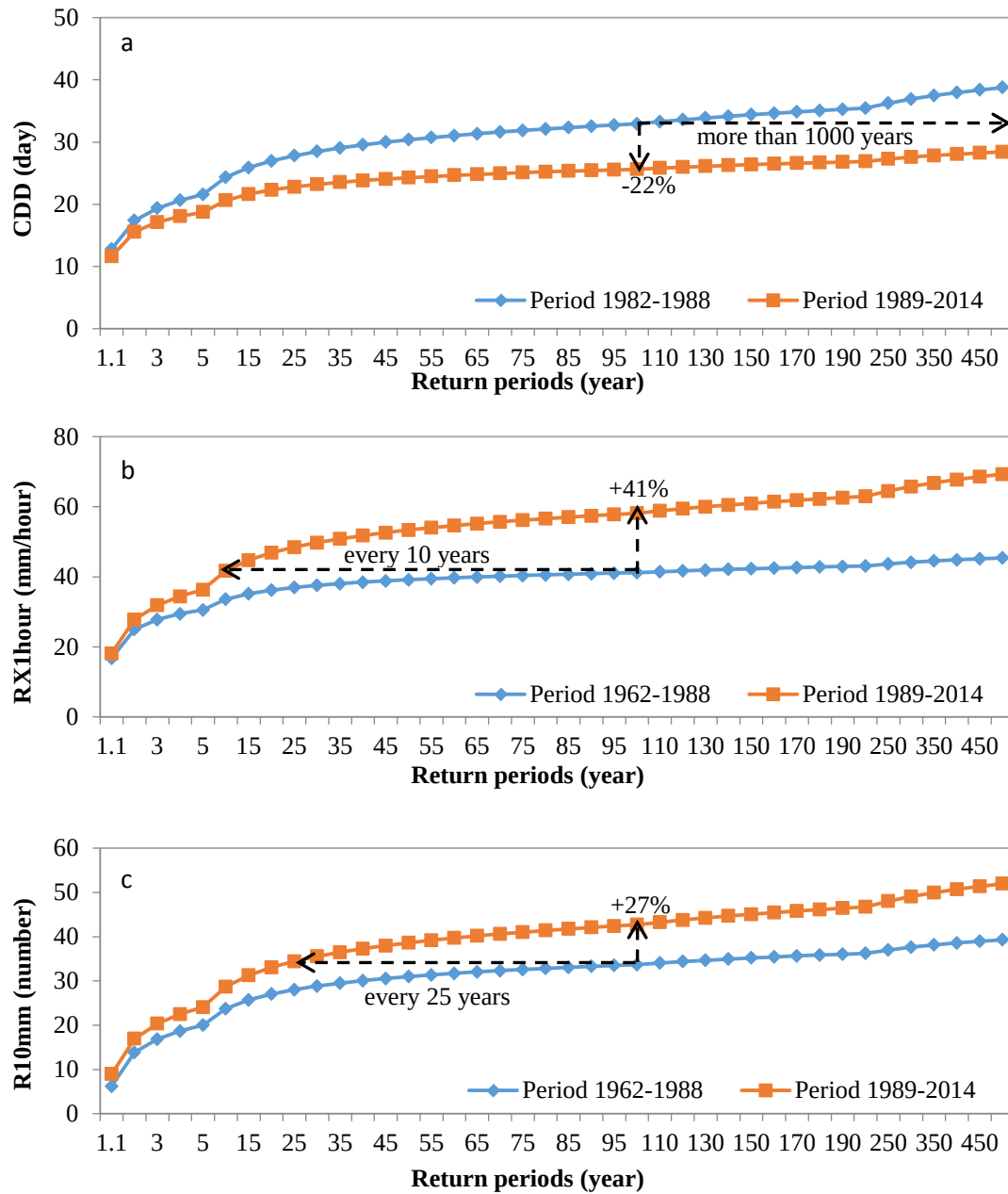
Figure 6-7 Annual inverse cumulative distribution functions of extreme precipitation indices: a) CDD, b) RX1hour, c) R10mm
