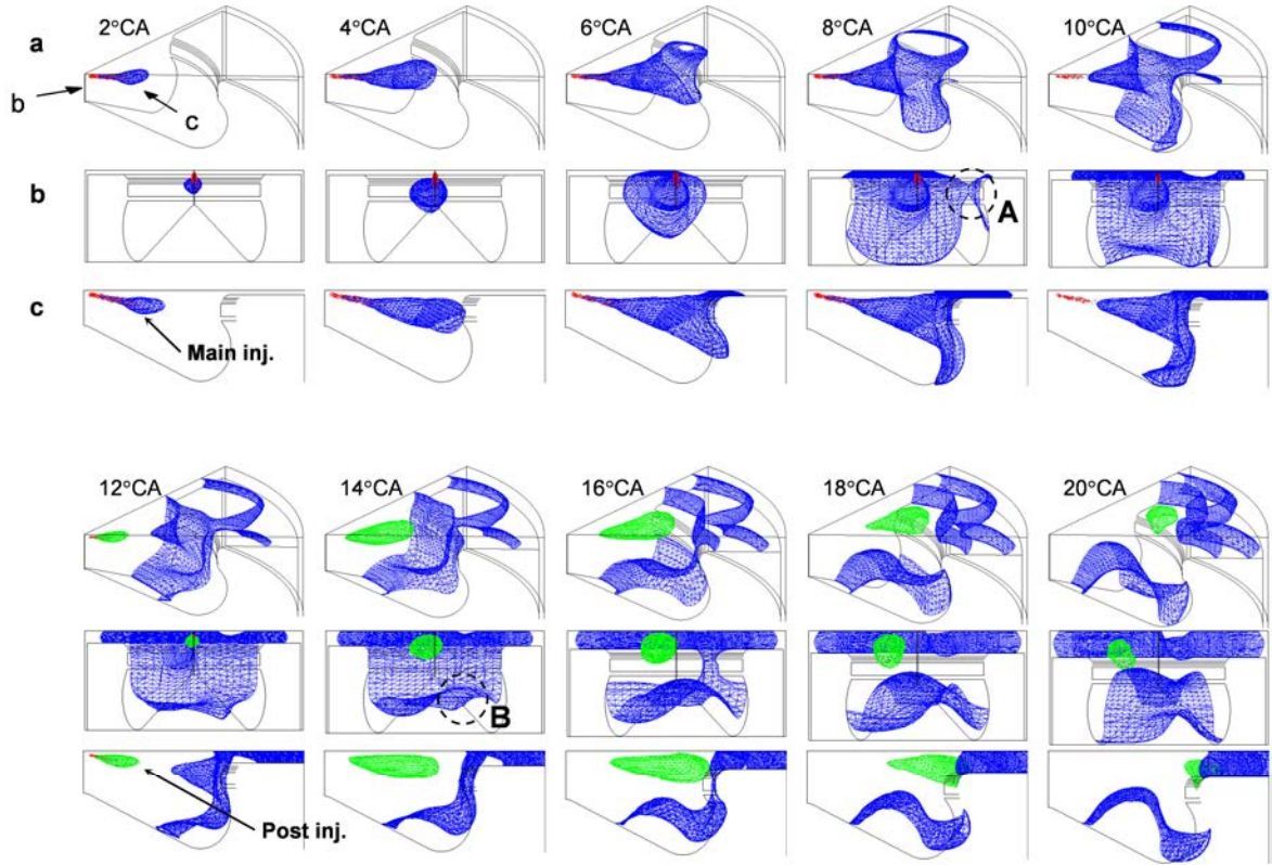
Fig. 4 Iso-surface of mixture fraction f_u=0.05 (Re55, 0.125 mm \times 7 holes nozzle, \theta_{\text{post}}=11^\circ\text{ATDC} )
