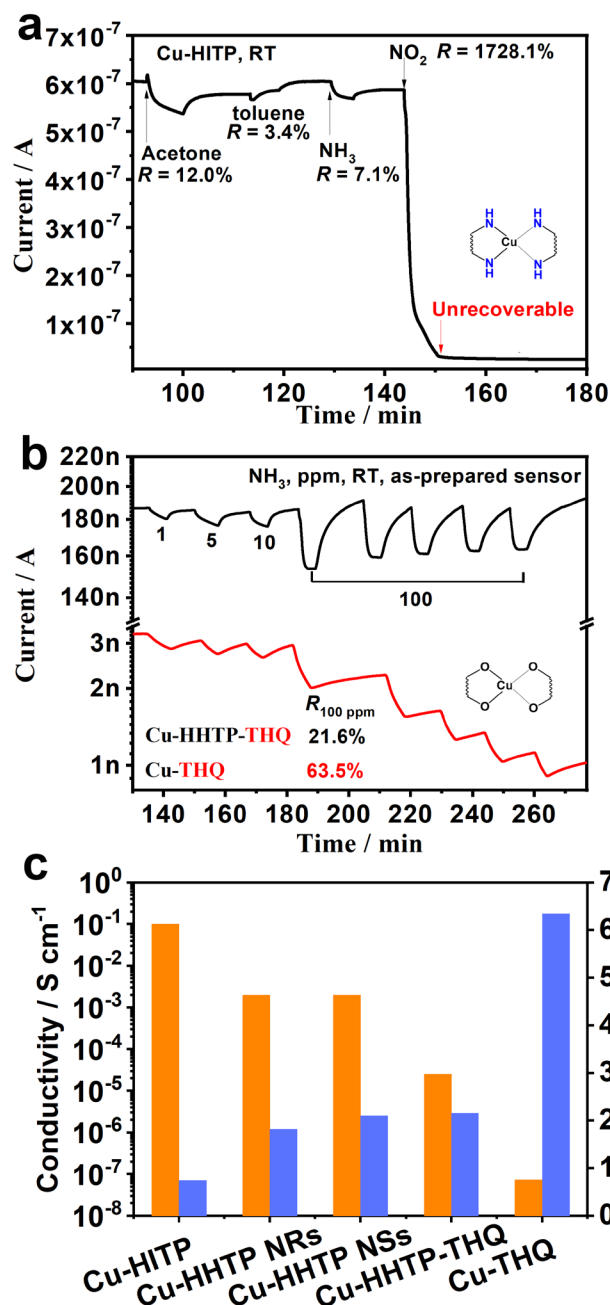
Fig. 6 (a) The dynamic sensing curve of Cu-HITP sensor toward typical reducing gases (acetone 1000 ppm, toluene 100 ppm, \text{NH}_3 100 ppm) and oxidizing gas ( \text{NO}_2 100 ppm); (b) dynamic sensing curves of the Cu-HHTP-THQ and Cu-THQ sensors toward \text{NH}_3 gases with different concentration; and (c) 2-probe pellet conductivity 35, 37, 39 and response values (100 ppm of \text{NH}_3 ) comparison of as-prepared cMOF sensors.
