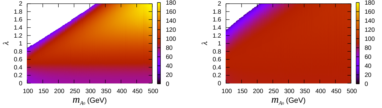
Figure 3: The lighter CP-even Higgs mass m_h . The horizontal axis is the mass of A^0 and the vertical axis is the coupling \lambda . The left panel is plotted with \tan \beta = 3 , while the right panel is done with \tan \beta = 10 .
