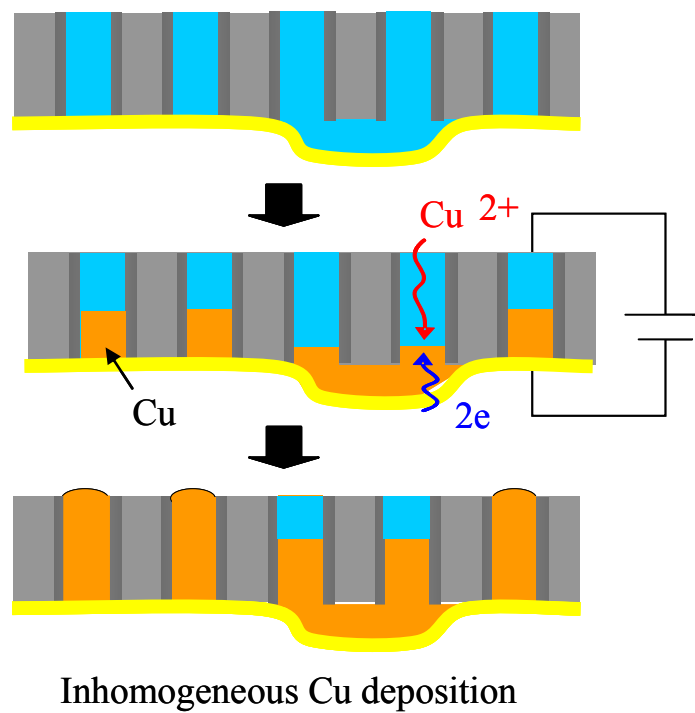
Fig.3.2 Uneven plating caused by insufficient contact of the seed layer.
