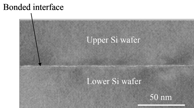
Fig.4.6 TEM photograph of Si wafers bonded interface.
