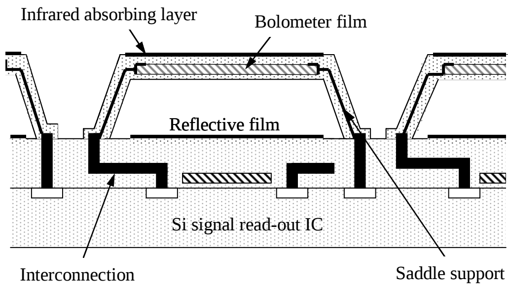
Fig.1.2 Bolometer type infrared sensor.
