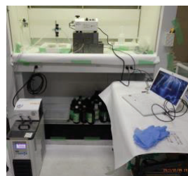
Fig. 2. Experimental set-up for separation of Lu-177 from Yb-176.
