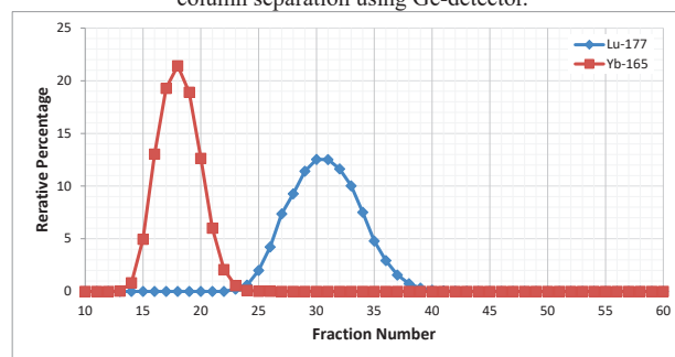
Fig. 2. Elution profile of extraction chromatography with an 11 mm \phi x 240 mmL column packed with LN2 resin measured with a Ge detector.
