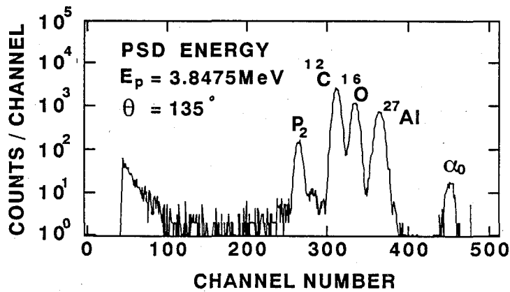
Fig. 4. Typical energy spectrum obtained with the PSD in the ^{27}\text{Al}(\text{p,p}) and ^{27}\text{Al}(\text{p},\alpha)^{24}\text{Mg} reactions. ^{12}\text{C} , ^{16}\text{O} and ^{27}\text{Al} indicate the elastic protons. \text{P}_2 shows inelastic protons by 2nd excitation of ^{27}\text{Al} , and \alpha_0 indicates the \alpha particles from ^{27}\text{Al}(\text{p},\alpha)^{24}\text{Mg} reaction.
